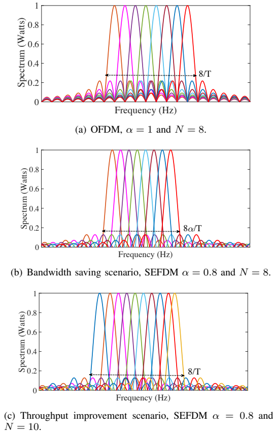
Fig. 3. OFDM and SEFDM Spectra for \alpha = 0.8, 1 .
