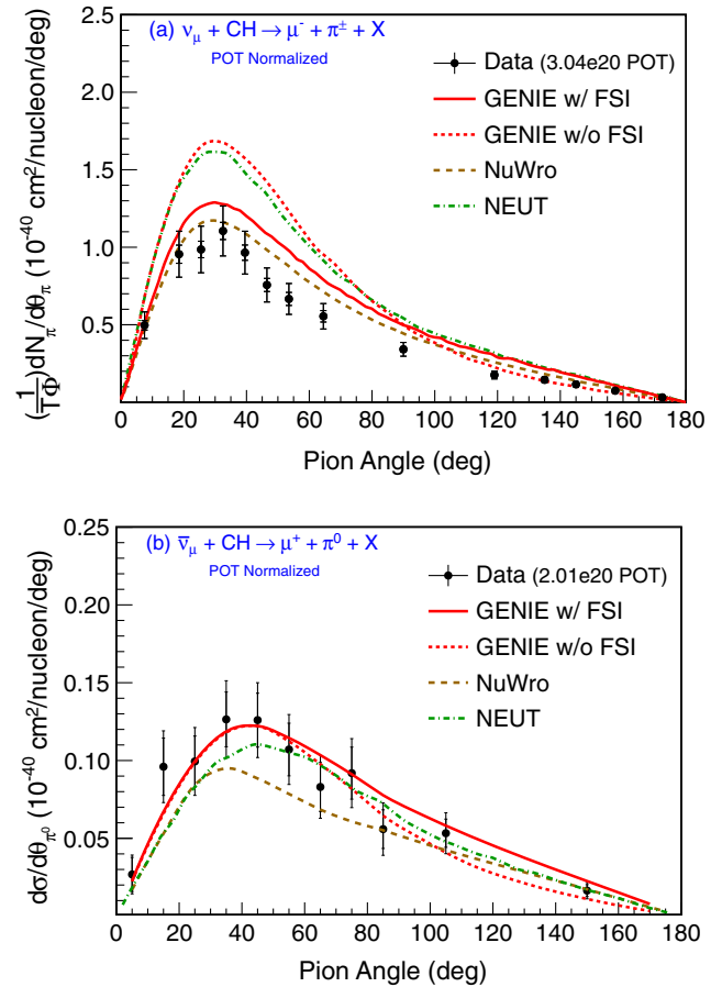
FIG. 16. Differential cross sections for the pion production angle with respect to the beam direction, d\sigma/d\theta_{\pi^\pm} , for the \nu_\mu -CC( \pi^+ ) (a) and \bar{\nu}_\mu -CC( \pi^0 ) (b) samples. As in Fig. 15, the data is compared to GENIE predictions without and with pion FSI effects included; marked improvement with the data is observed when pion FSI is taken into account (solid-line distributions).
