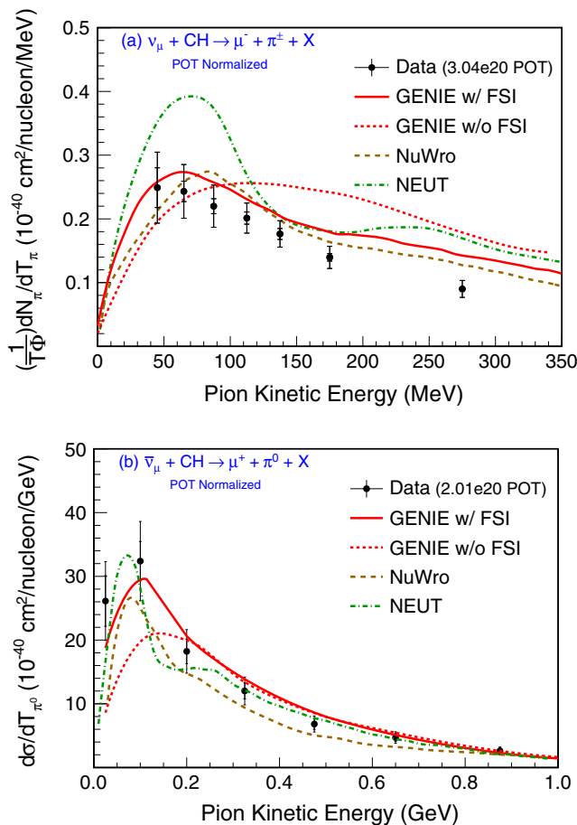
FIG. 15. Differential cross sections for pion kinetic energy, d\sigma/dT_{\pi^\pm} , for the \nu_\mu -CC( \pi^+ ) (a) and \bar{\nu}_\mu -CC( \pi^0 ) (b) samples. The data (solid circles) are compared to GENIE predictions neglecting versus including pion FSI (dashed vs solid-line histograms). Improved descriptions for shapes of the pion spectra are obtained with FSI effects included in the simulations.
