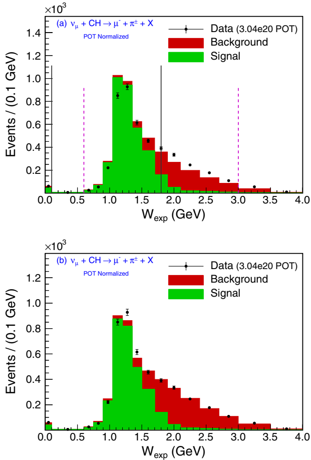
FIG. 3. The W_{\text{exp}} spectrum for the \nu_\mu -CC( \pi^+ ) sample comparing the data (solid points) to the Monte Carlo simulation (histograms) before (a) and after (b) the fit over the region between the vertical dashed lines in the upper plot. The Monte Carlo prediction is the sum of signal template (green online) and background template (red online) contributions. The analysis selects a signal-dominated sample (between the vertical solid lines) by requiring W_{\text{exp}} < 1.8 GeV.
