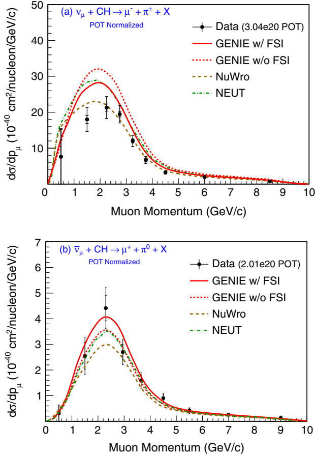
FIG. 7. Differential cross sections as a function of the muon momentum for the \nu_\mu (a) and \bar{\nu}_\mu (b) pion production samples. Data are shown as solid circles. The inner (outer) error bars correspond to statistical (total) uncertainties. The solid (dashed) distributions are GENIE predictions with (without) FSI. Also shown are predictions for the NuWro and NEUT event generators.
