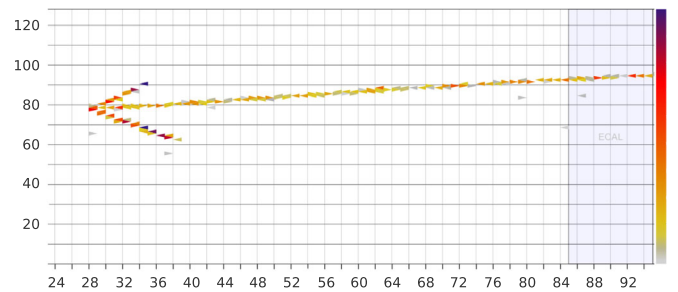
FIG. 1. Neutrino data event of the \nu_\mu -CC( \pi^+ ) sample from the top view. The neutrino enters from the left. The primary vertex occurs in the central scintillator tracking region; the muon traverses the downstream ECAL and HCAL regions and projects into the MINOS near detector (downstream, not shown). The event is a candidate for the final state \mu^- \pi^+ p . The X and Y axis labels show the module and strip numbers. The color (online) linear scale (0–10 MeV) indicates the amount of energy deposited in the strips.
