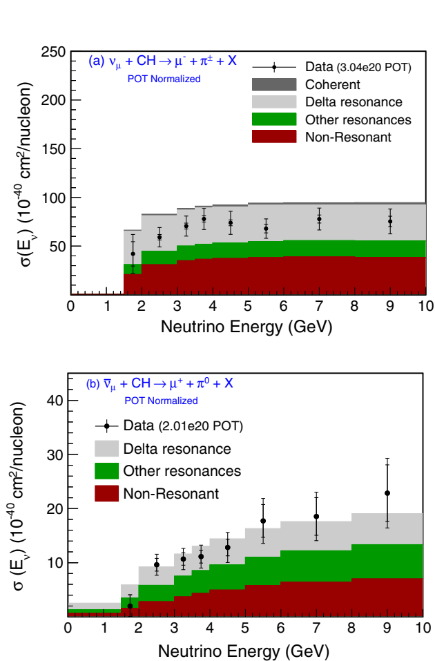
FIG. 11. Component reaction processes in GENIE cross-section predictions for the \nu_\mu -CC( \pi^+ ) (a) and \bar{\nu}_\mu -CC( \pi^0 ) (b) samples. Stacked histograms (bottom to top) show the contributions from (i) pion nonresonance processes, (ii) N^* states above the \Delta(1232) , and (iii) \Delta(1232) resonance production.
