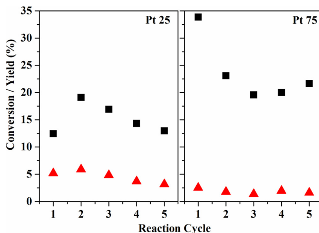
Fig. 9. Glycerol conversion (■) and H 2 yield (▲) for 2% Pt/Al 2 O 3 catalysts produced at 25 °C and 75 °C. Reaction conditions: 240 °C, PAr = 42 bar, 1000 rpm, 10 wt% glycerol, 60 mg catalyst, 2 h reaction time.
