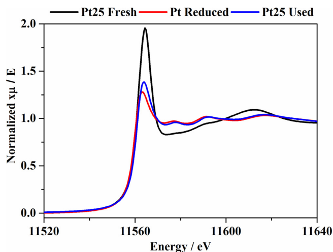
Fig. 12. Normalised XANES spectra of Pt25 in the fresh, reduced and used states.
