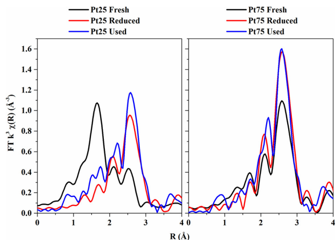
Fig. 11. EXAFS analysis of Pt25 and Pt75 catalysts in the fresh, reduced and used states.
