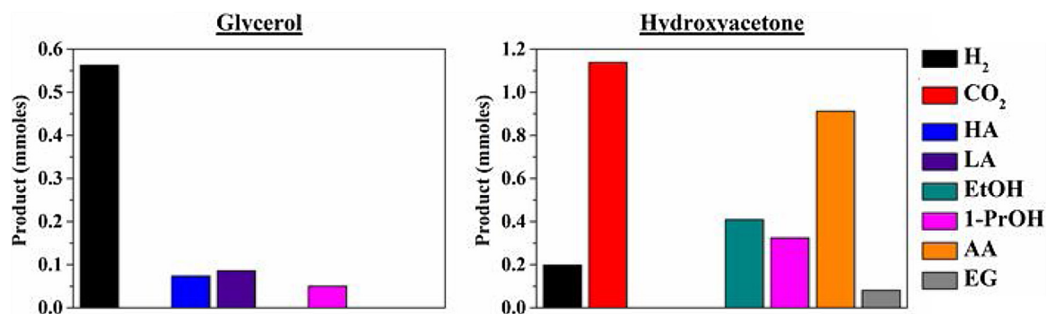
Fig. 8. Product formation from glycerol and hydroxyacetone over Al 2 O 3 . Reaction conditions: 240 °C, PAr = 42 bar, 1000 rpm, 10 wt% reactant, 60 mg catalyst, reaction time = 2 h for glycerol, 1 h for hydroxyacetone.
