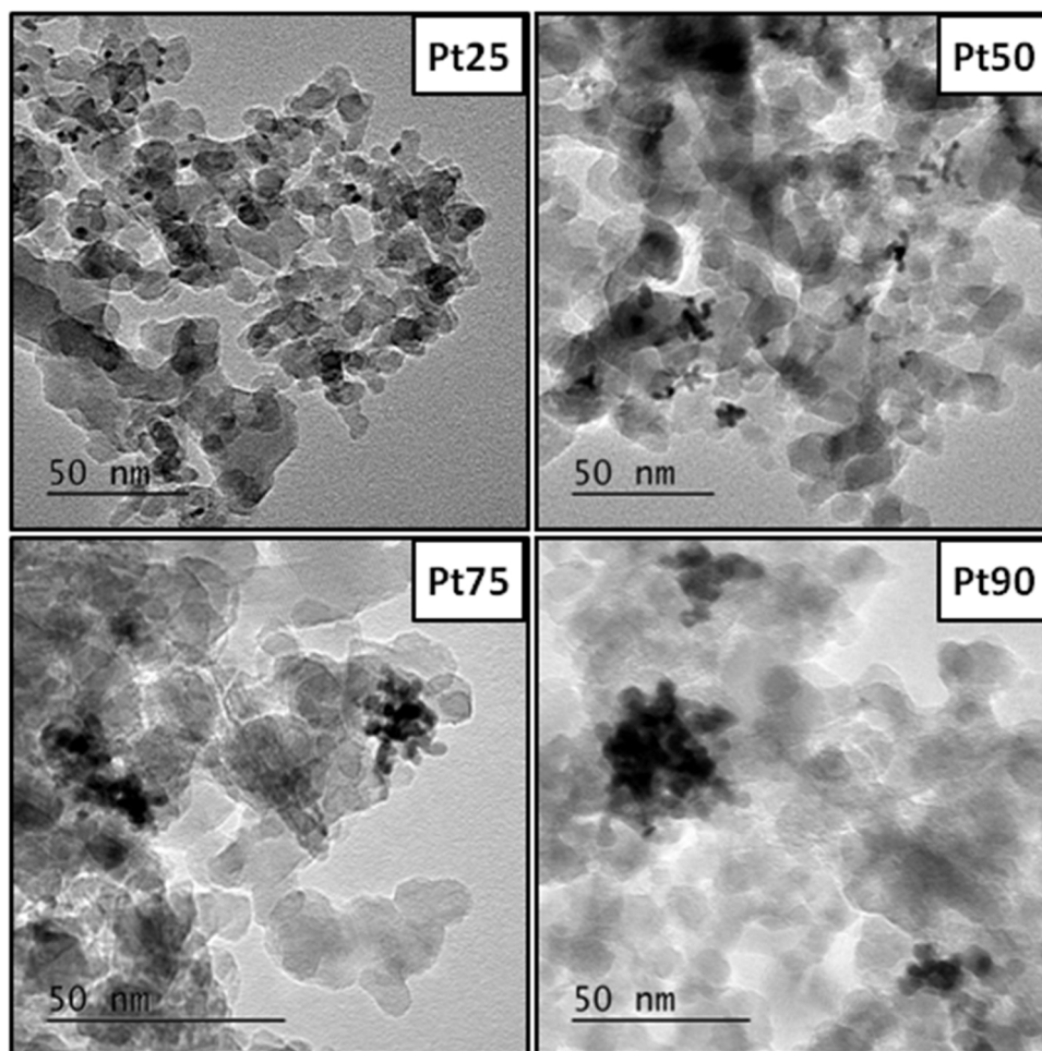
Fig. 3. TEM images of catalyst samples Pt25 (top left), Pt50 (top right), Pt75 (bottom left) and Pt90 (bottom right) at 50 nm scale.
