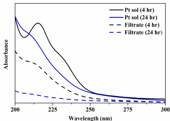
Fig. 1. UV–vis spectra of Pt sols after reduction with \text{NaBH}_4 for 4 h and 24 h, plus the respective filtrated solutions after immobilisation on \text{Al}_2\text{O}_3 .
