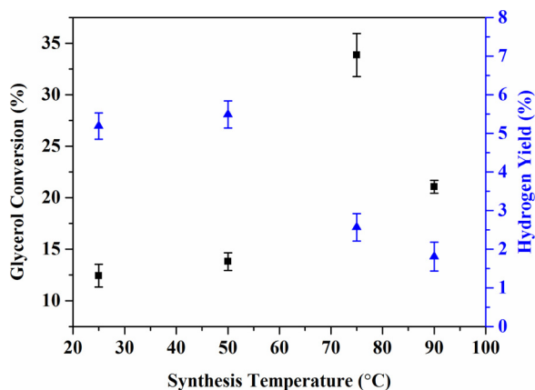
Fig. 4. Glycerol conversion (■) and H 2 yield (▲) for 2% Pt/Al 2 O 3 catalysts produced at different colloidal reduction temperatures. Reaction conditions: 240 °C, P Ar = 42 bar, 1000 rpm, 10 wt% glycerol, 60 mg catalyst, 2 h reaction time.
