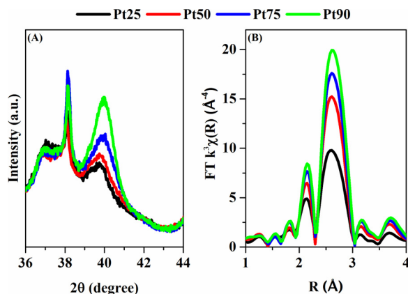
Fig. 2. XRD (A) and EXAFS (B) analysis of 2% Pt/Al 2 O 3 catalysts produced at different colloidal reduction temperatures, black – Pt25, red – Pt50, blue – Pt75, green – Pt90 (For interpretation of the references to colour in this figure legend, the reader is referred to the web version of this article).
