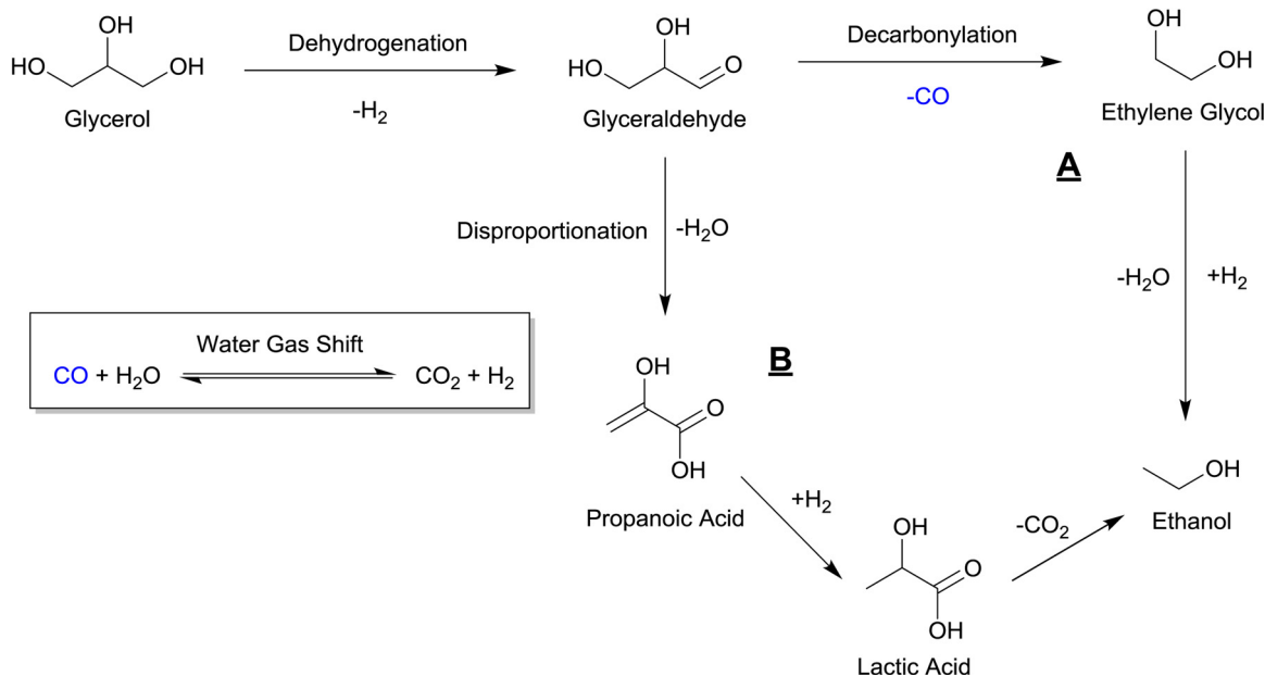
Scheme 1. Proposed reaction pathway for APR of glycerol – Route 1.
