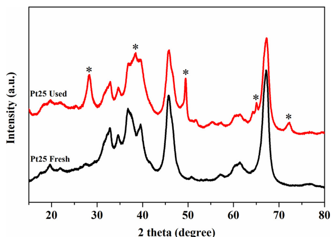
Fig. 14. XRD patterns of Pt25 before (fresh) and after (used) aqueous-phase glycerol reforming reaction.
