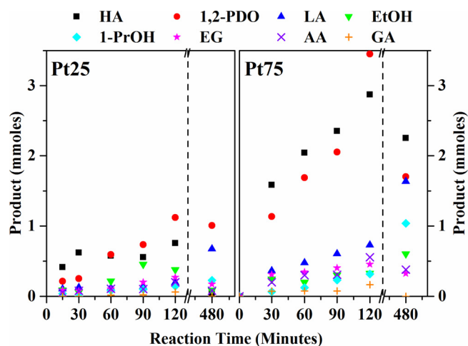
Fig. 6. Major liquid products formed from APR of glycerol using Pt25 and Pt75 catalysts over various reaction times. Reaction conditions: 240 °C, P_{Ar} = 42 bar, 1000 rpm, 10 wt% glycerol, 60 mg catalyst.
