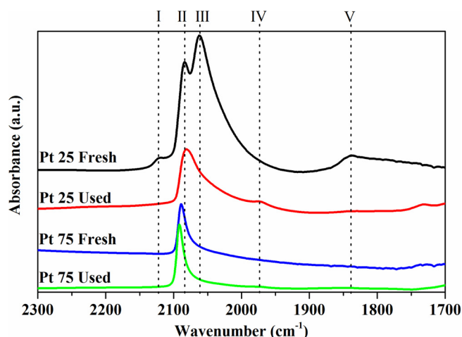
Fig. 10. CO adsorption coverage of Pt25 and Pt75 catalysts before and after one reaction cycle of 2 h.
