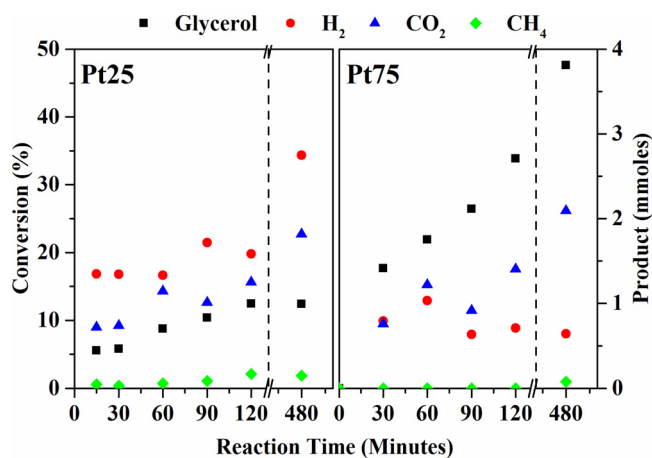
Fig. 5. Glycerol conversion and gas products from APR of glycerol using Pt25 and Pt75 catalysts over various reaction times. Reaction conditions: 240 °C, P Ar = 42 bar, 1000 rpm, 10 wt% glycerol, 60 mg catalyst.
