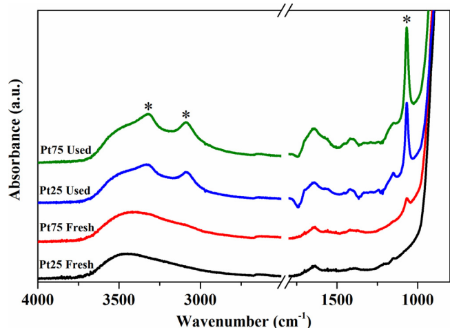
Fig. 13. ATR-FTIR Spectra of Pt25 and Pt75 samples before and after aqueous-phase glycerol reforming reaction.
