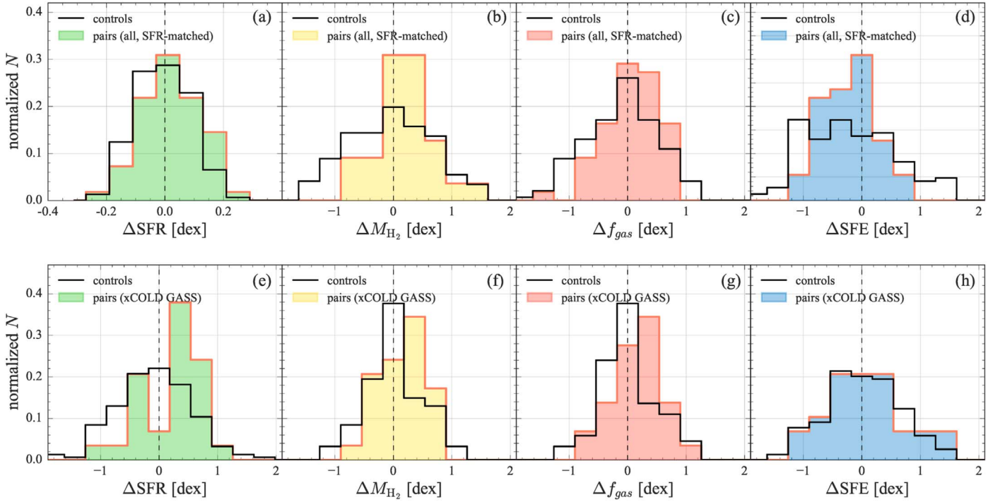
Figure 10. (a)–(d) Normalized distribution of \Delta SFR, \Delta M_{\text{H}_2} , \Delta f_{\text{gas}} , and \Delta SFE. The plot is similar to that of Figures 4(e)–(h), but we additionally match the galaxies and control sample in SFR. Therefore, the values along the x-axis in panel (a) are considerably smaller than those in the other panels. Galaxies in pairs with high sSFR are not considered here (see text for details) due to the lack of suitable controls. With SFR as one of the matching parameters, the enhancements of \Delta M_{\text{H}_2} and \Delta f_{\text{gas}} are still present in galaxies in pairs. The SFE seems to be suppressed in galaxies in pairs after matching in SFR. This is because SFE is SFR divided by M_{\text{H}_2} by definition. (e)–(h) The plots are made using the data values that generated Figures 4(e)–(h) (without matching in SFR), but only galaxies in pairs from xCOLD GASS are shown. Since the control galaxies are drawn from xCOLD GASS as well, any potential bias induced by different selection criteria for galaxies in pairs (Section 2) and any uncertainty in the conversion from CO(2–1) to CO(1–0) intensities are removed. It is evident that the distributions of \Delta SFR, \Delta M_{\text{H}_2} , and \Delta f_{\text{gas}} still peak at higher values with respect to the controls when only the xCOLD GASS galaxies in pairs are considered.
