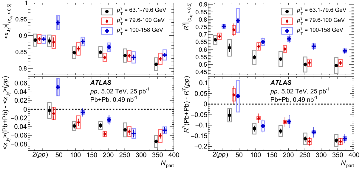
Fig. 8. Summary of (left) the mean jet-to-photon p_T ratio ( x_{J\gamma} ) and (right) the total per-photon jet yield R^{\gamma} , calculated in the region x_{J\gamma} > 0.5 . The values are presented as a function of the mean number of participating nucleons N_{\text{part}} in top panels. Each colour and symbol represents a different p_T^{\gamma} interval, where the lowest and highest intervals are displaced horizontally for clarity. The points plotted at N_{\text{part}} = 2 correspond to pp collisions. The bottom panels show the difference between the Pb + Pb centrality selection and pp collisions. Boxes show the total systematic uncertainty while the vertical bars represent statistical uncertainties.
