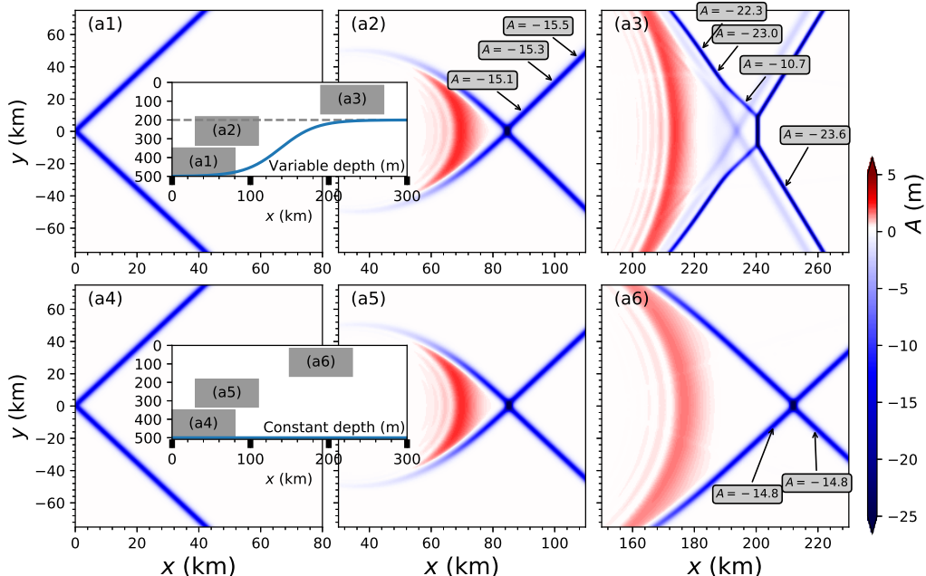
FIGURE 5. For EXP1, panels (a1-a3) are selected to exhibit the evolution of wave patterns in the case of shoaling topography at times t = 0, 12, 42 hours respectively. In contrast, panels (a4-a6) are for the case of constant topography at times t = 0, 12, 30 hours respectively. Note that as the waves propagate faster in the constant-depth case, the snapshot is not an exact one-to-one match. The aspect ratio of every panel is the same, that is x \times y = 80 \times 150 km, and the corresponding depth of every panel is indicated by insets.
