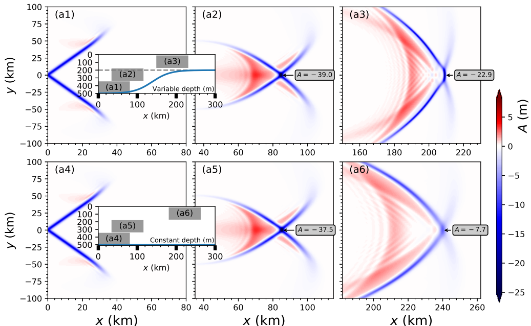
FIGURE 9. The layout is the same as in figure 5 but the aspect ratio of every panel is x \times y = 80 \times 200 \text{ km} here. The set-up is the same as that in EXP1, except that an envelope is imposed on the initial V-shape wave.
