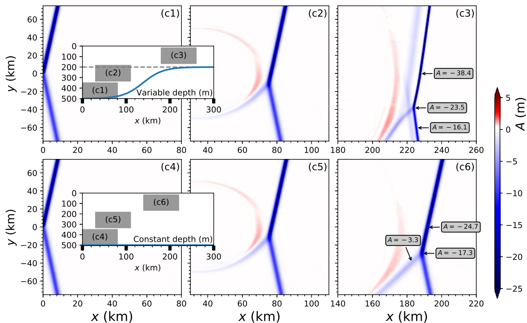
FIGURE 8. The layout is the same as in figure 5, but for EXP3.
