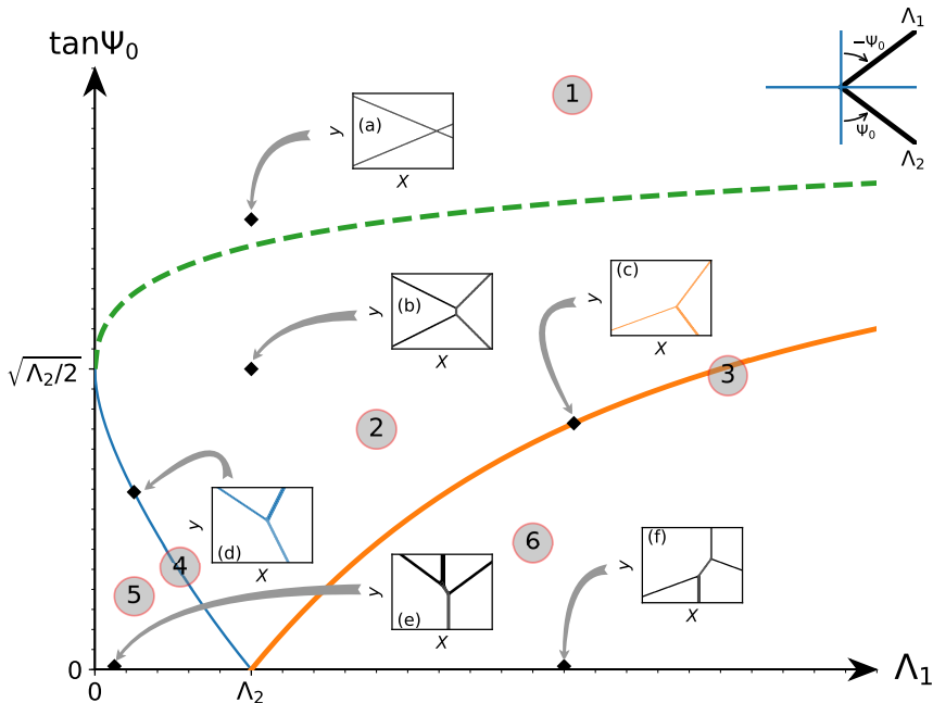
FIGURE 2. The initial V-shape wave (2.23) is depicted in the right upper corner. In the constant-coefficient KP equation (2.14), with the amplitude of the lower branch \Lambda_2 fixed, the developed wave patterns which evolve corresponding to the amplitude of the upper branch \Lambda_1 and slope \tan \Psi_0 are shown. The evolution regime can be divided into six regions, and specially region 3 and 4 are just along the thick solid line (in the colour of orange) and thin solid line (in blue) respectively. The green dashed line is given by \sqrt{2\Lambda_1} + \sqrt{2\Lambda_2} = 2 \tan \Psi_0 , the thick solid line is given by \sqrt{2\Lambda_1} - \sqrt{2\Lambda_2} = 2 \tan \Psi_0 , and the thin solid line is given by \sqrt{2\Lambda_2} - \sqrt{2\Lambda_1} = 2 \tan \Psi_0 . A similar figure is also given in Oikawa et al. (2010).
