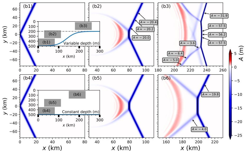
FIGURE 7. The layout is the same as in figure 5, but for EXP2.
