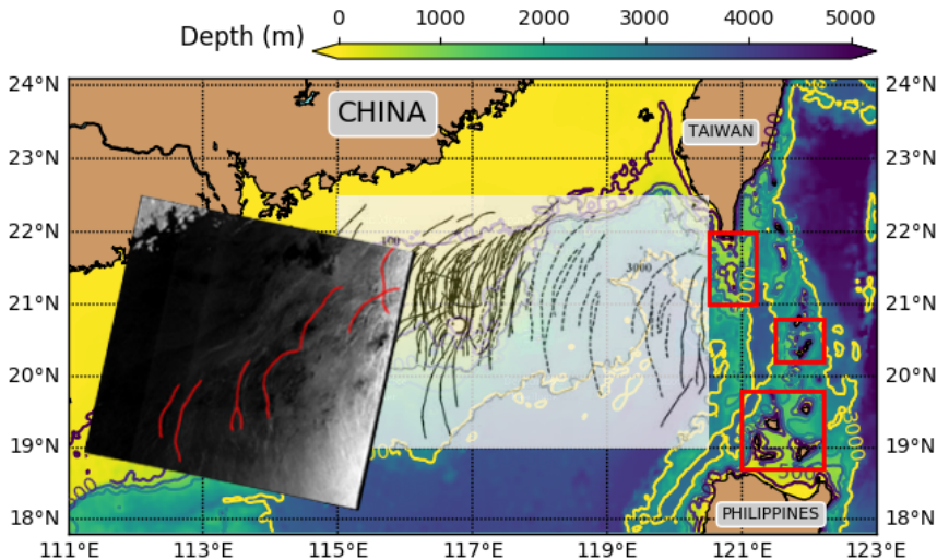
FIGURE 1. The bathymetry of the South China Sea. Three red rectangles indicate the potential generation sites, see Guo and Chen (2014). The transparent inset, adopted from Zhao et al. (2004), shows the existence of the multi-wave ISW packets (solid line) and single-wave ISW packets (dashed line), which is a collection of the satellite images acquired from 1995 to 2001. An Envisat-1 Advanced SAR satellite image on 02:20 UTC, 31-07-2010 is also imposed, where some wave crestlines are accentuated in red lines.
