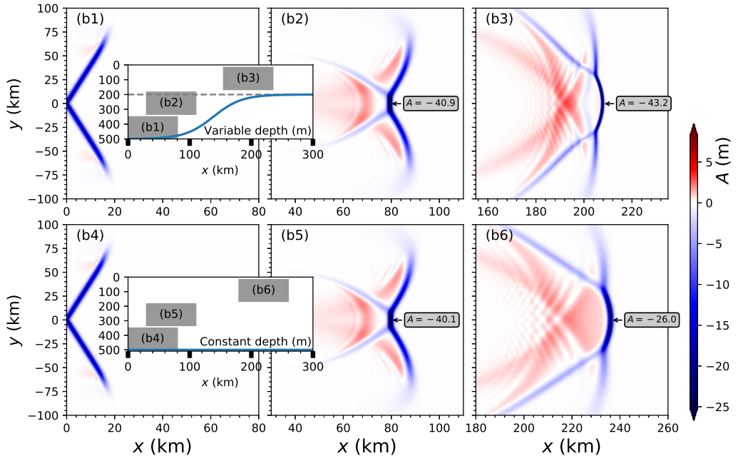
FIGURE 10. The layout is the same as in figure 5 but the aspect ratio of every panel is x \times y = 80 \times 200 \text{ km} here. The set-up is the same as that in EXP2, except that an envelope is imposed on the initial V-shape wave.
