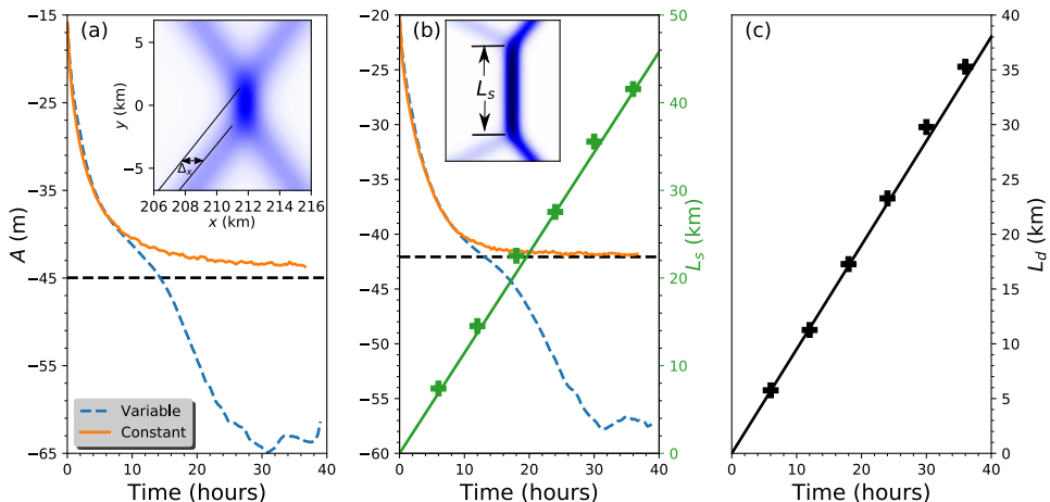
FIGURE 6. (a) In EXP1, the time series of the leading wave amplitude along y = 0 for the cases of both varying and constant topography. The inset is a zoom-in of panel (a6) in figure 5. (b) In EXP2, the time series of the leading wave amplitude along y = 0 for the cases of both varying and constant topography. The inset is a zoom-in of panel (b6) in figure 7. The other scale shows the length of the intermediate Mach stem L_s predicted by the theory (green solid line) and the numerical simulations (green plus sign). (c) The downward distance L_d varying with time in EXP3 is shown and the solid line is the theoretical result, while the plus sign is from numerical simulations.
