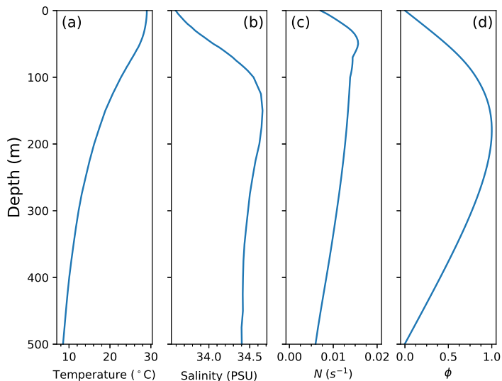
FIGURE 4. The vertical profiles of the temperature (a), salinity (b), buoyancy frequency N (c) and the corresponding mode-1 modal function \phi (d) from equations (2.2) and (2.3).
