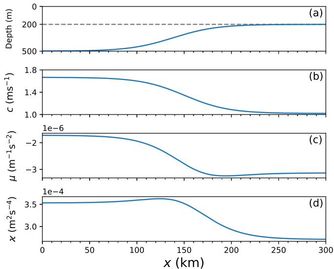
FIGURE 3. The y -independent bathymetry h (a); the linear phase speed c (b); the nonlinear coefficient \mu (c); the dispersive coefficient \chi (d).
