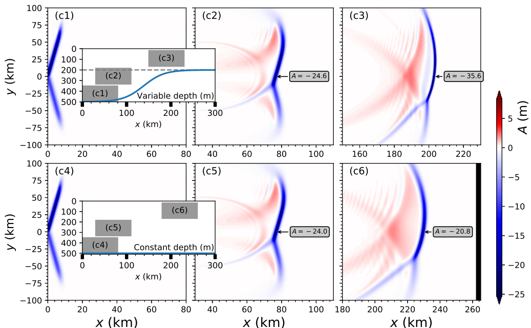
FIGURE 11. The layout is the same as in figure 5 but the aspect ratio of every panel is x \times y = 80 \times 200 \text{ km} here. The set-up is the same as that in EXP3, except that an envelope is imposed on the initial V-shape wave.
