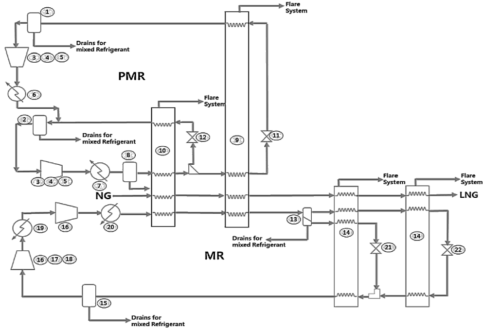
Figure 6: Flow diagram of LNG MR liquefaction cycle
