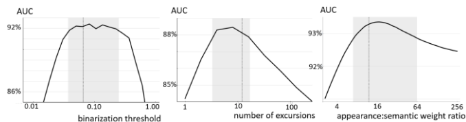
Fig. 14. Effect of hyper-parameters on performance. Left: appearance anomaly detection as a function of the binarization threshold. Middle: semantic anomaly detection as a function of the number of excursions from the mean. Right: combined anomaly performance as a function of the ratio of weights applied to the appearance and semantic scores.
