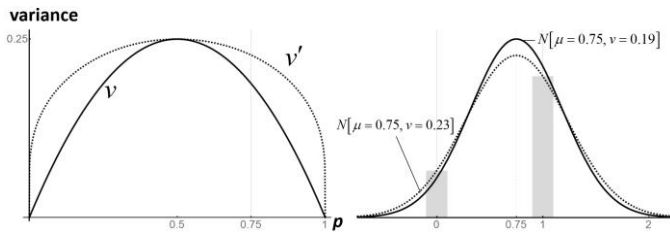
Fig. 8. Compares the naïve (solid) and adjusted (dotted) Gaussians used to model distributions of binary values. Left: variance of the modelling Gaussian as a function of the sample mean. Right: the modelling Gaussians (curves) for a distribution (grey bars) of binary values with mean 0.75. The bars coincide with the adjusted Gaussian at variate values 0 and 1.
