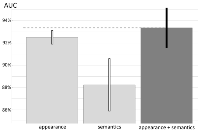
Fig. 11. Performance of combined vs. individual approaches to anomaly detection. Same details as Fig. 9.
