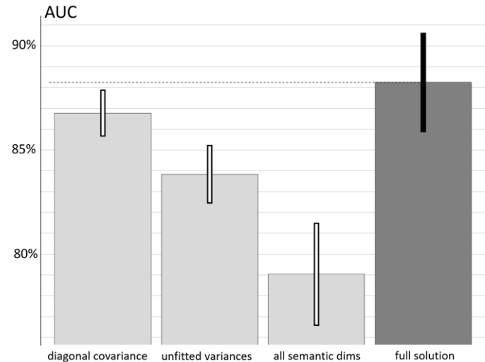
Fig. 10. Performance of different approaches to anomaly detection based on real-valued semantic vectors. Same details as Fig. 9.
