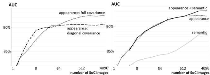
Fig. 13. Effect of training set size on performance. Left plot compares two schemes for appearance anomalies. Right plot compares individual and combined anomaly detection schemes.
