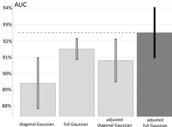
Fig. 9. Performance of different approaches to AD based on binarized appearance vectors. In all cases, the normal population was 4096 SoC parcels, and testing was on staged-threat parcels and held-out SoC parcels. Wide grey bars show mean performance using different random training and test sets with 95% confidence intervals (not shown) of less than \pm 1\% . The best method (‘adjusted full Gaussian’) is shown with a darker bar and a 95% confidence interval showing the uncertainty of its absolute performance given the finite pool of training and test data. The other hollow error bars shows the 95% confidence interval of the relative performances of the sub-optimal methods compared to the best method; none cross the dashed line indicating that they are significantly worse.
