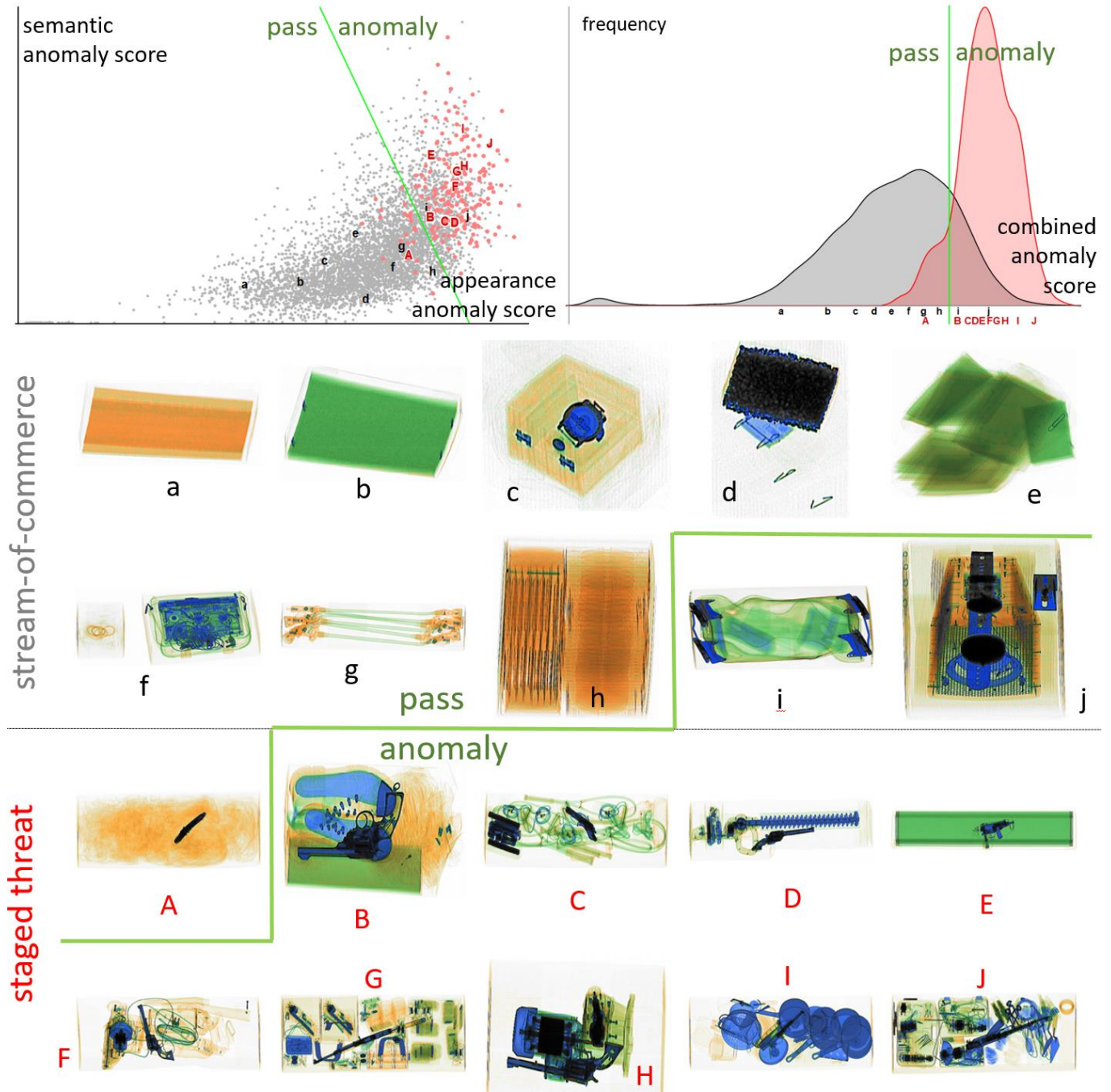
Fig. 12. Illustration of the combined scheme for anomaly detection. In all panels the green line marks the same hard threshold, images below this threshold 'pass', images above are considered 'anomalies'. The threshold is set to catch 90% of the staged-threat images, but triggers false alarms for 18% of SoC images. Top-left: appearance scores vs. semantic scores for SoC (grey) and threat (pink) images. Top-right: histograms of the combined scores, same colour scheme as left. Bottom four rows: example SoC and threat images. Letters labelling each image correspond to locations in the top row plots.
