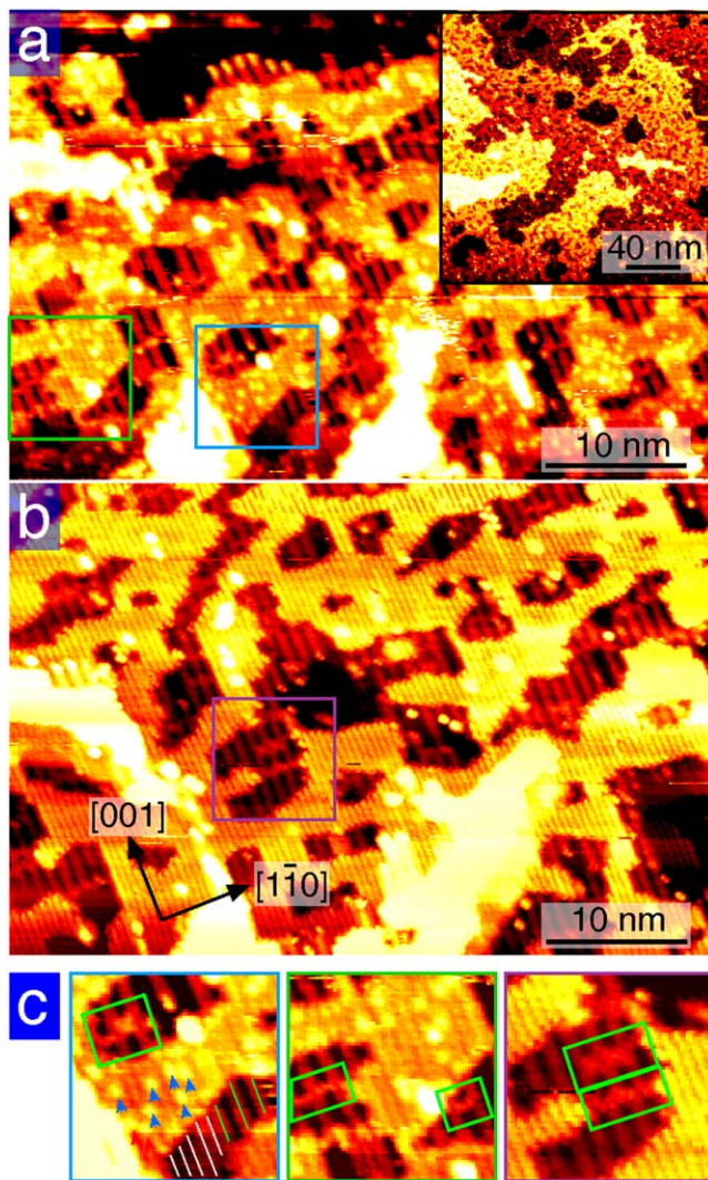
Figure 9. STM images recorded from an outer beam region of the e-beam exposed surface (3 keV, 0.65 \text{ mA cm}^{-2} for 40 min, e-exp 2) after annealing the sample to \sim 850 \text{ K} . (a) and (b) both 50 \times 33 \text{ nm}^2 (1.83 V, 0.36 nA) show a flat mixed 1 \times 1/1 \times 2 terminated surface. The insert in (a) 200 \times 200 \text{ nm}^2 shows a large scale image which displays the retention of typical step structures. (c) 8 \times 8 \text{ nm}^2 . Enlarged areas from (a) and (b) including (blue box) individual point defects (i.e. \text{O}_{\text{vac}} or \text{OH}_{\text{br}} , blue arrows) on a 1 \times 1 area, and a mixed 1 \times 1/1 \times 2 terrace (white and green lines respectively). 1 \times 2 reconstructed regions with single links and crosslinks are highlighted with green boxes.
