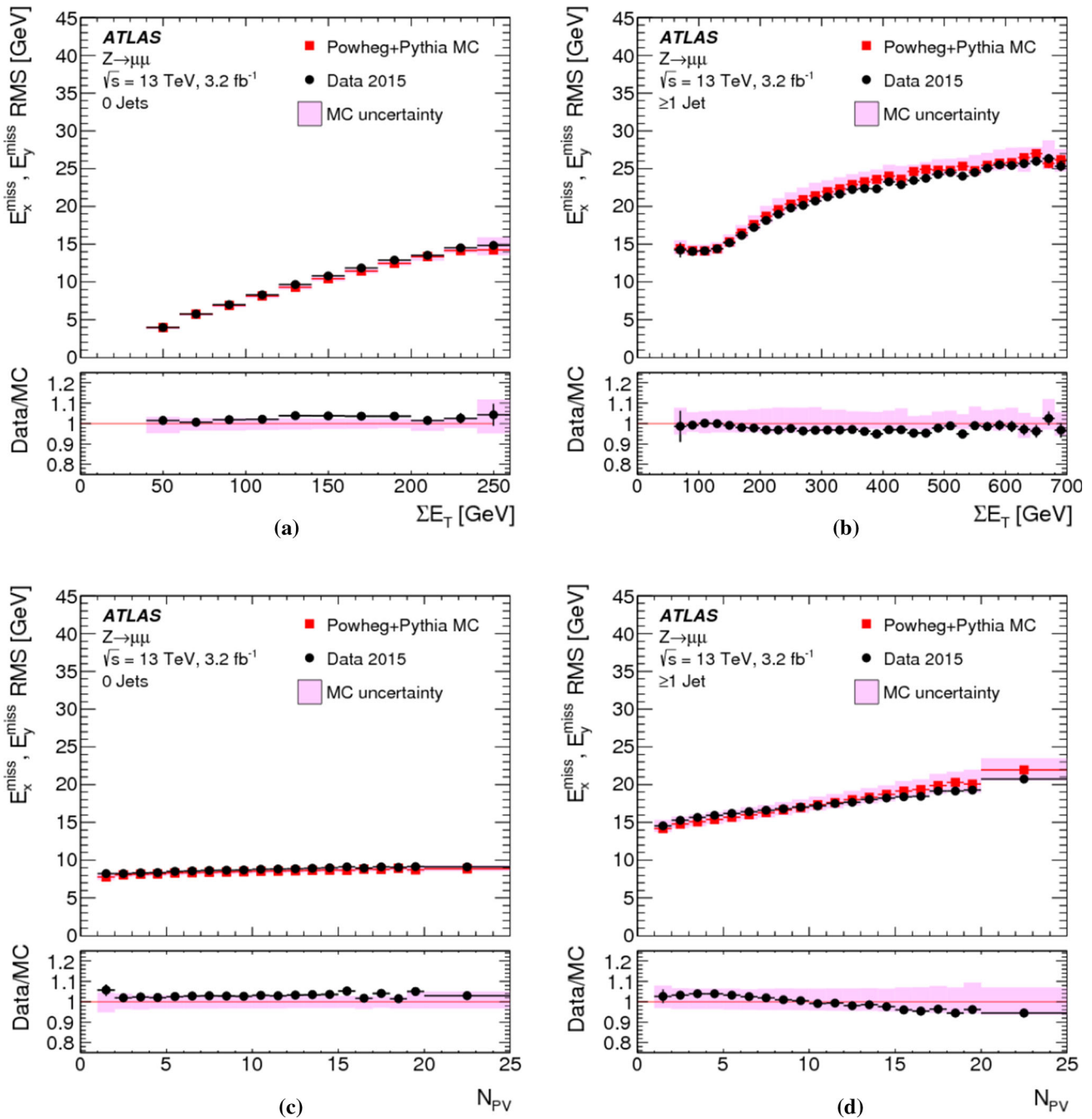
Fig. 8 The E_T^{\text{miss}} resolution \text{RMS}_{x(y)}^{\text{miss}} determined for a an exclusive Z \rightarrow \mu\mu sample without jets with p_T > 20 \text{ GeV} ( N_{\text{jet}} = 0 ) and for b an exclusive sample with at least one jet above this threshold ( N_{\text{jet}} \geq 1 ), as a function of \Sigma E_T in data and MC simulations. The dependence of
