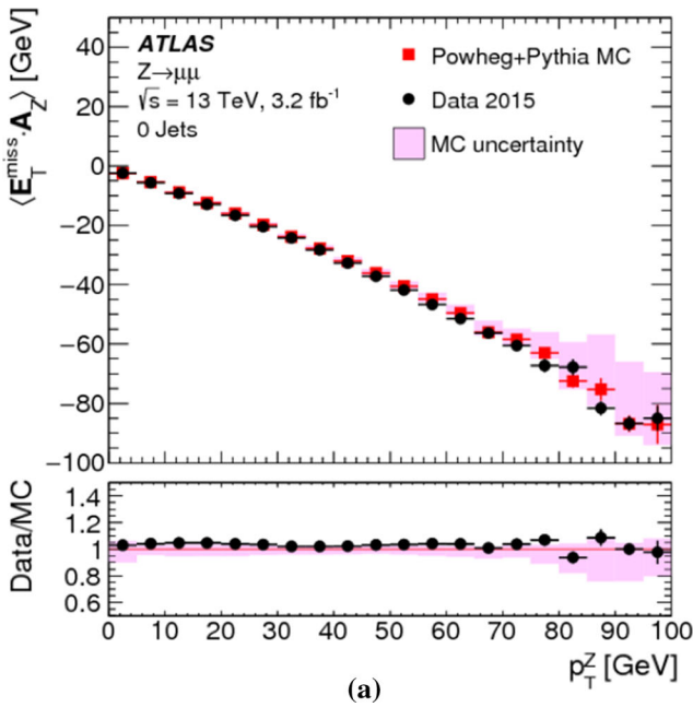
Fig. 4 The average projection of E_T^{\text{miss}} onto the direction A_Z of the Z boson's transverse momentum vector p_T^Z , as given in Eq. (10), is shown as a function of p_T^Z = |\mathbf{p}_T^Z| in Z \rightarrow \mu\mu events from a the N_{\text{jet}} = 0 sample and from b the inclusive sample. In both cases data are compared to MC simulations. The ratio of the averages from data and MC simula-
