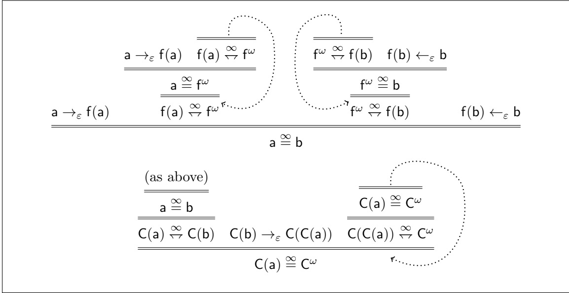
Figure 5: An example of infinitary equational reasoning, deriving C(a) \overset{\infty}{\equiv} C^{\omega} in the TRS \mathcal{R} of Example 6.2. Recall Notation 4.1.
