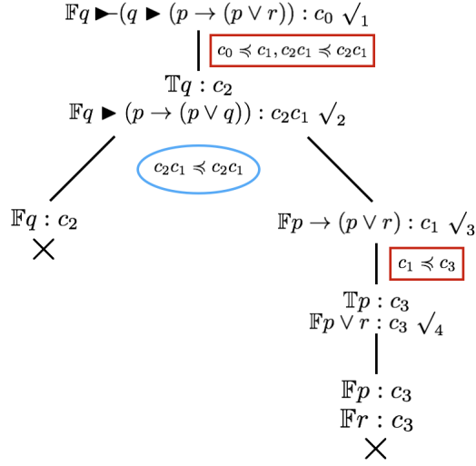
Figure 11: A tableau proof of q \blacktriangleright (q \blacktriangleright (p \rightarrow (p \vee r)))
