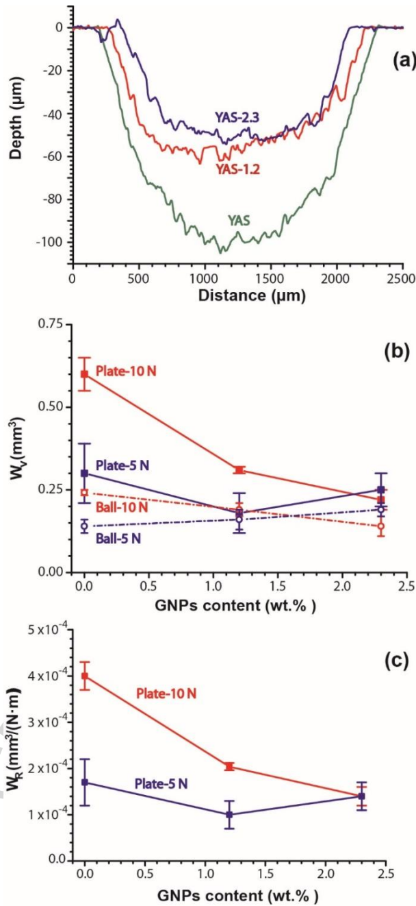
Fig. 3. (a) 2D profiles of representative wear tracks of the different coatings tested at 10 N; (b) Wear volume ( W_v ) versus GNPs content of the plates (coatings) and the balls tested at 5 and 10 N; and (c) wear rate ( W_R ) versus GNPs content of the coatings tested at 5 and 10 N.
