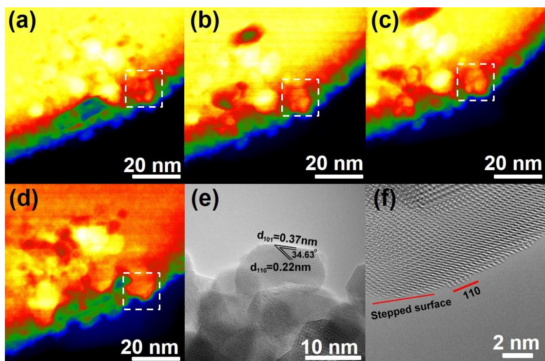
Fig. 2 HAADF images (in false color) of single-crystalline BiOCl exposed by e^- beam (average dose rate: ca. 0.5 e/A^2 \cdot s ) for 5 min (a), 10 min (b), 20 min (c) and 40 min (d) respectively. The dashed squares in (a-d) indicate the growth and coalescence of Bi NPs. (e) depicts the HRTEM image of an individual bismuth nanoparticle and (f) shows the aberration-corrected HRTEM image near a (110) surface plane with a stepped surface.
