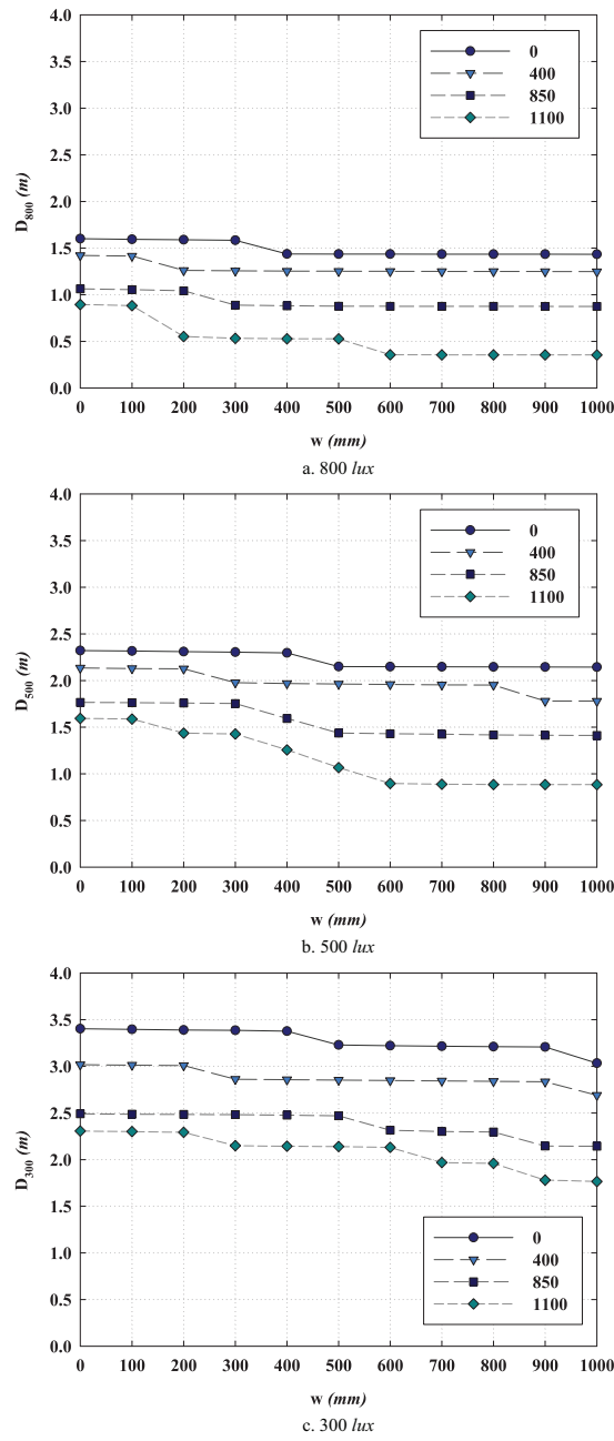
Fig. 9 D values of the cube with different widths for different illuminance contours
