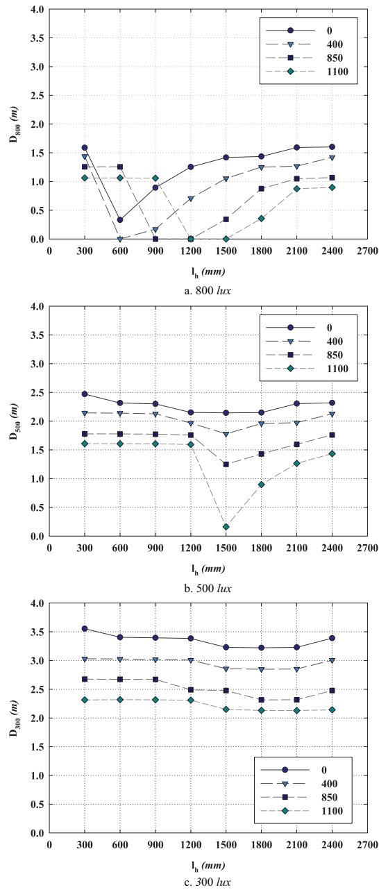
Fig. 5 D values of the cube at different position heights for different illuminance contours
