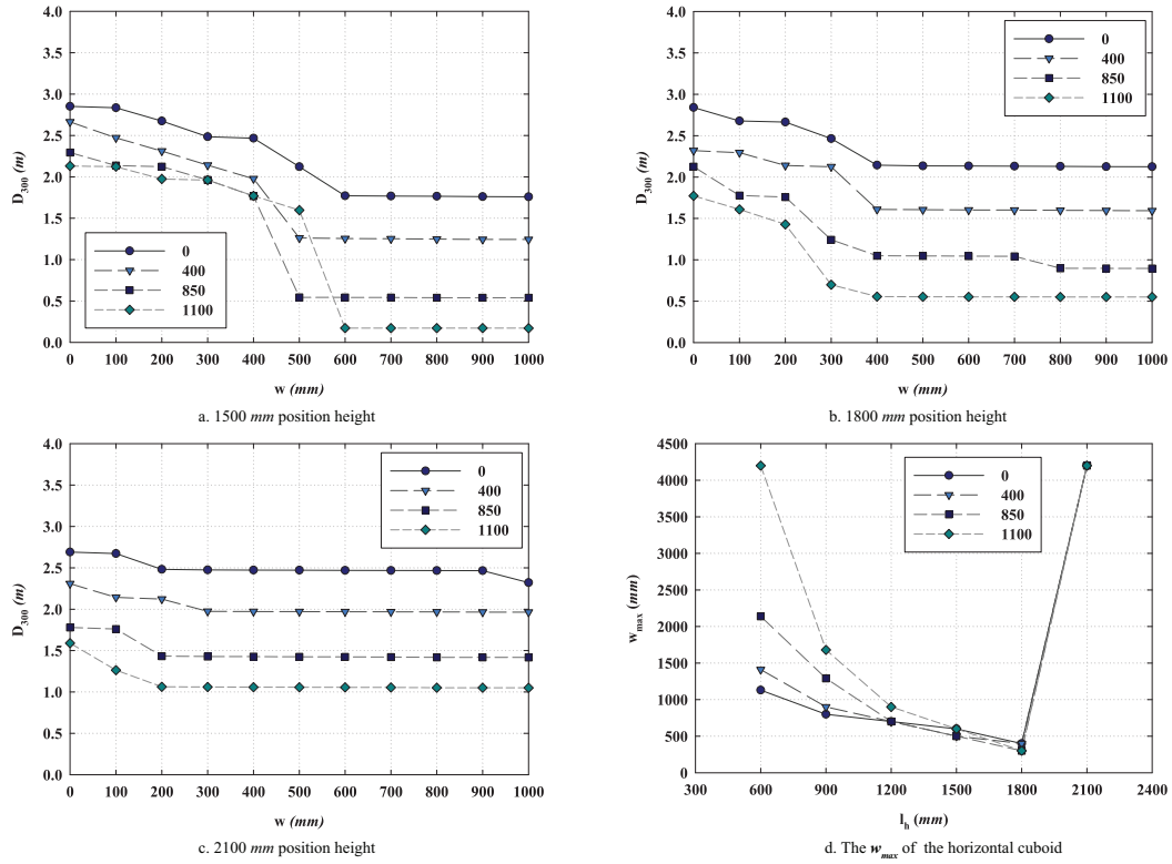
Fig. 12 D values of the horizontal cuboid with different widths at different position heights for the 300 lux illuminance contour and the w_{max} of the horizontal cuboid for the 300 lux illuminance contour on the 850 mm high working plane
