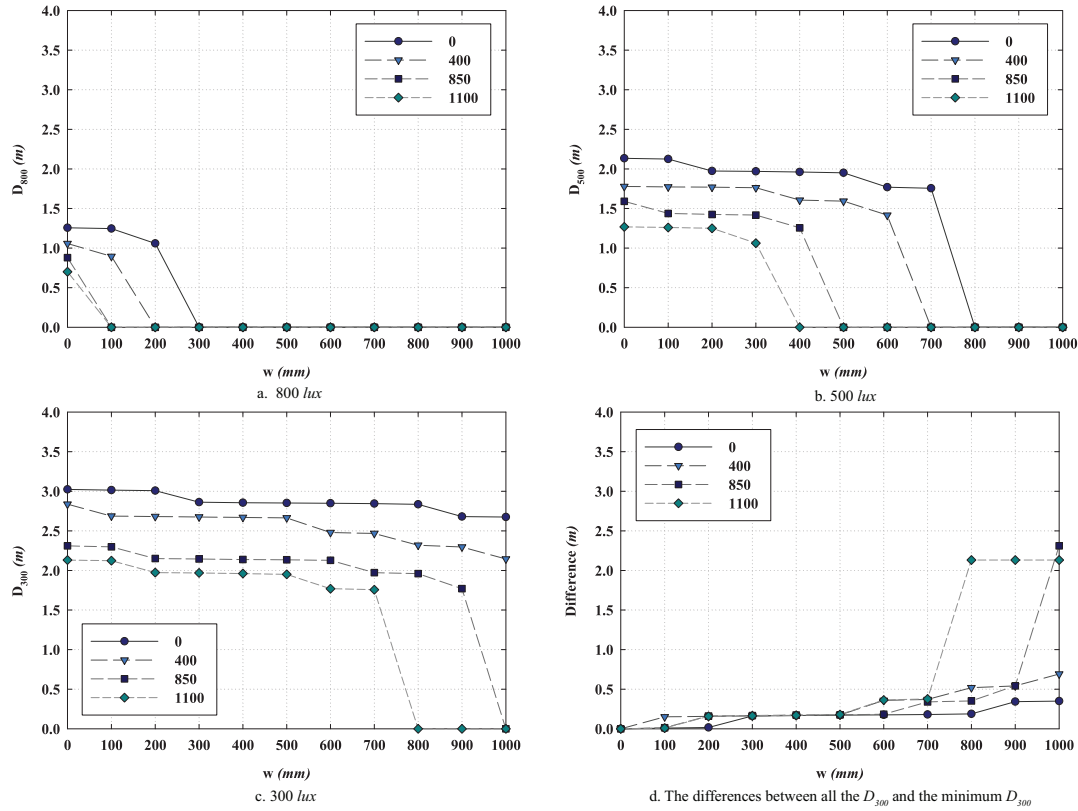
Fig. 10 D values of the vertical cuboid with different widths for different illuminance contours and the differences between all the D_{300} values and the minimum D_{300}
