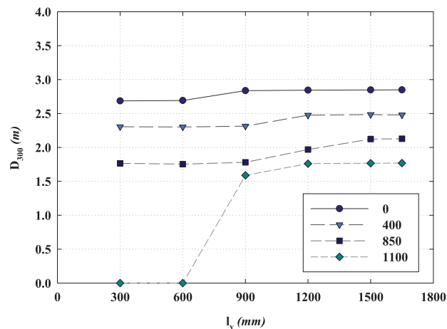
Fig. 7 D of the vertical cuboid at different horizontal positions for the 300 lux illuminance contour
