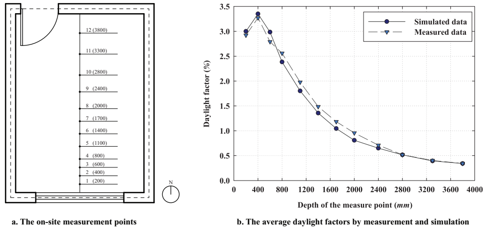
Fig. 2 The on-site measurement points and the average daylight factors by measurement and simulation
