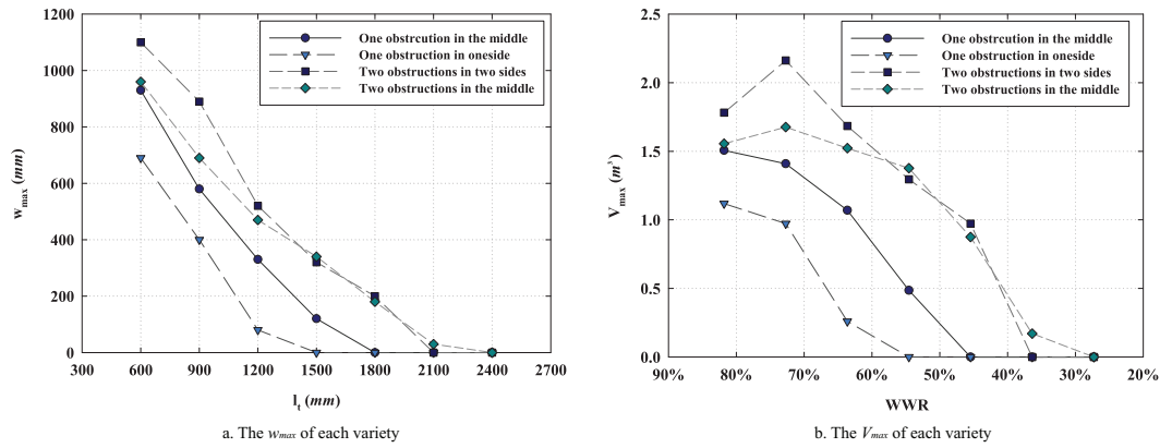
Fig. 11 The w_{max} , V_{max} of each simulation variety for the 300 lux illuminance contour on the 850 mm high working plane
