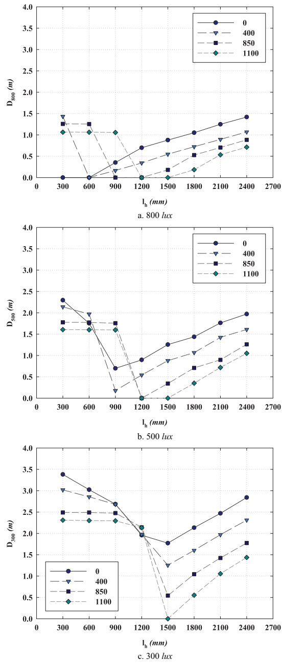
Fig. 8 D values of the horizontal cuboid at different position heights for different illuminance contours
