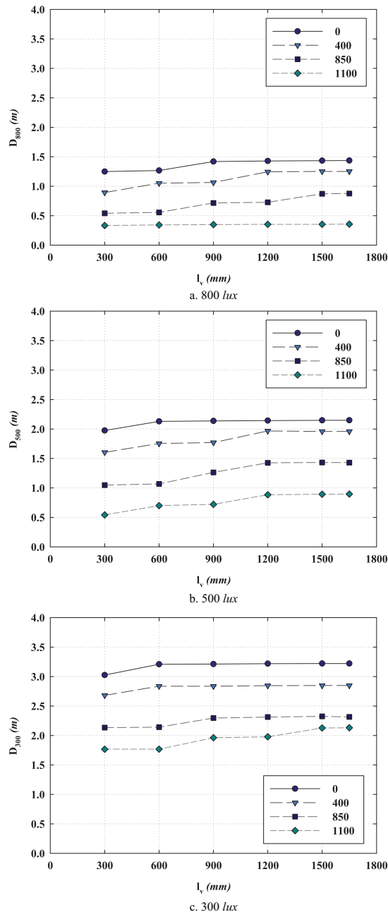
Fig. 6 D values of the cube at different horizontal positions for different illuminance contours
