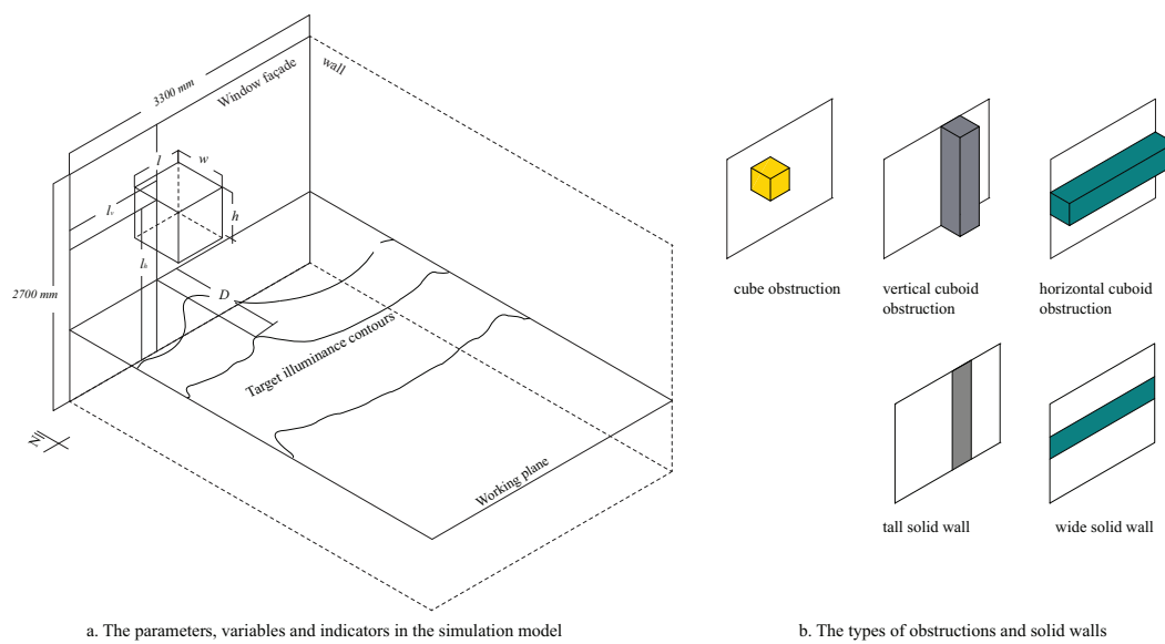
Fig. 3 The model and obstruction types in the simulation
