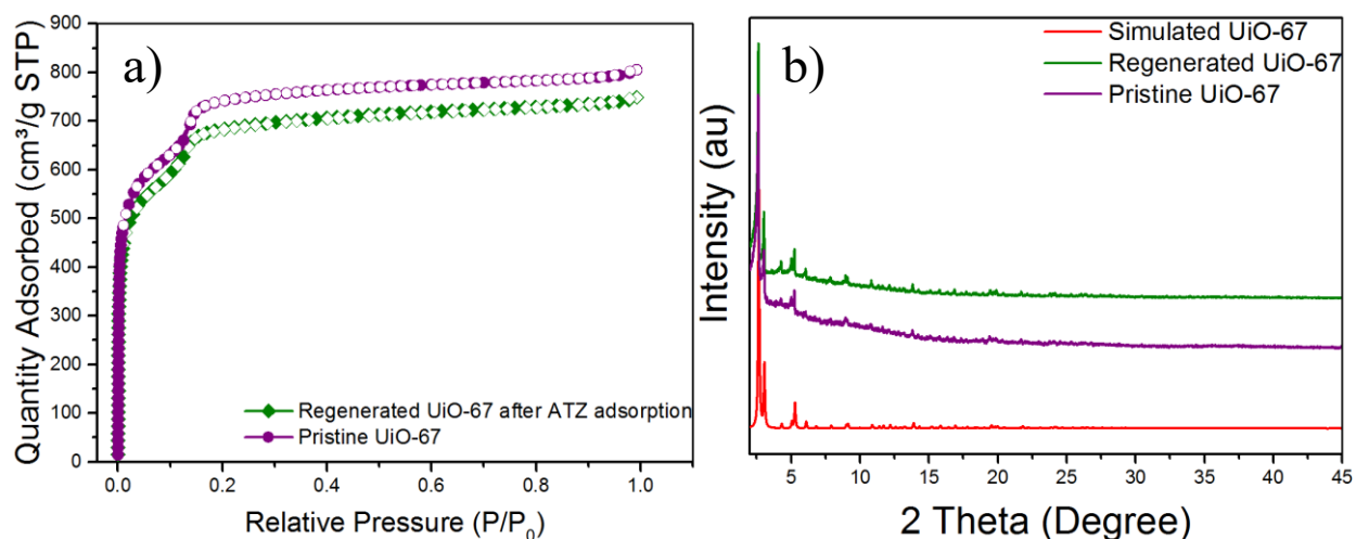
Figure 7. (a) N_2 adsorption-desorption isotherms of prepared UiO-67 and regenerated UiO-67 in acetone followed by thermally activated and (b) PXRD patterns of starting UiO-67 before adsorption of atrazine, regenerated after atrazine adsorption and the simulated PXRD pattern of UiO-67 is also included for comparison.
