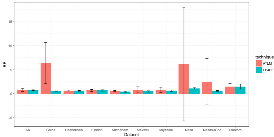
Fig. 1: RQ 2.2. Robustness to Different Data Splits (requirement 8) : Mean (height) and standard deviation (bar) of RE^* (over 30 runs) achieved by ATLM and LP4EE per dataset. The red dotted line represents the RE^* threshold value 1.
