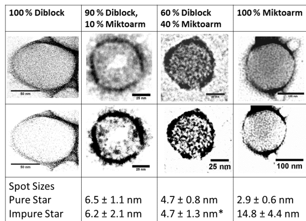
Figure 4: TEM micrographs, original and with enhanced contrast with spot sizes for polymersomes for varying PMPC-PDPA diblock to PMPC/PDPA-Mal-PEG Miktoarm star polymer composition. The contrast of the images has been enhanced to emphasize the presence of patches on the vesicle surface. *On a 50/50 mixture for impure star.
