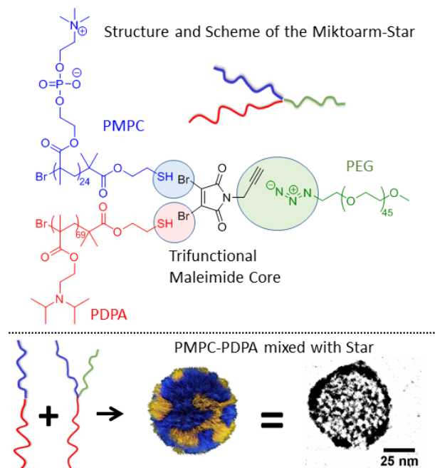
Figure 1: Scheme of the miktoarm star, including the click reactions used to synthesise it. PMPC (blue) and PDPA (red) are attached using thiol/dibromomaleimide conjugation, while PEG (green) is clicked on using CuAAC chemistry. If self-assembled together with a PMPC-PDPA diblock, patchy polymersomes evolve.
