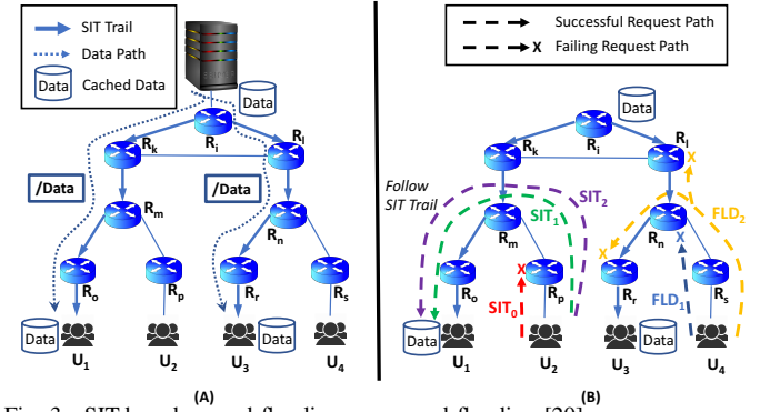
Fig. 3. SIT-based scoped flooding vs. scoped flooding [20].
