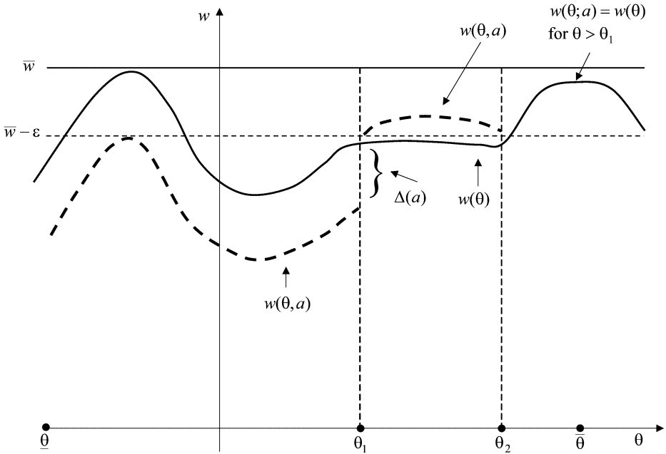
FIGURE 3.—The continuation value function: the down variation.
