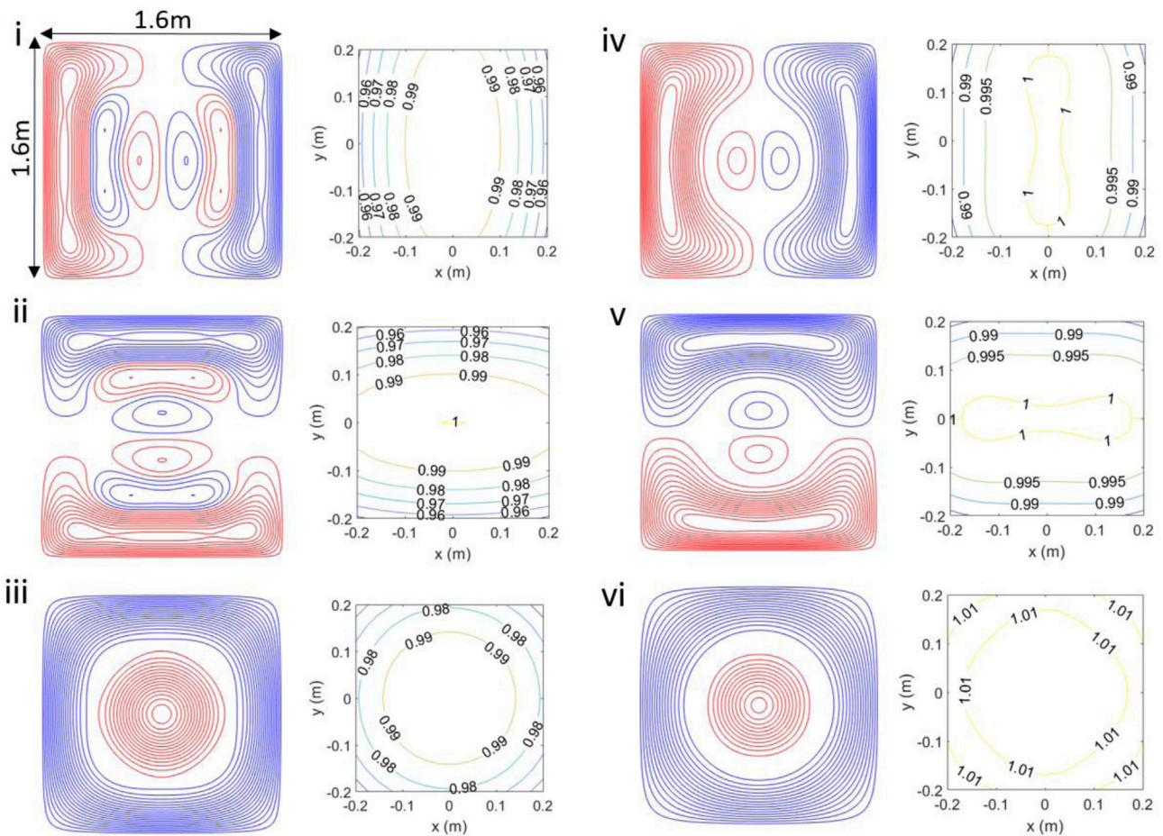
Fig. 4. Wire paths and field or field gradient contours for the: i) B_x , ii) B_y , iii) B_z , iv) dB_x/dz , v) dB_y/dz , vi) dB_z/dz coils. Red and blue denote wires with opposite senses of current flow. The contours of the field (i-ii) or field gradient (iv-vi) in the plane at z = 0 m, for |x|, |y| < 0.2 m ( z = 0.02 m, for |x|, |y| < 0.2 m for the dB_z/dz coil) are shown. The fields were normalised to the value at the centre of the two planes (or a value positioned off-centre where the field gradient is zero at the centre).
