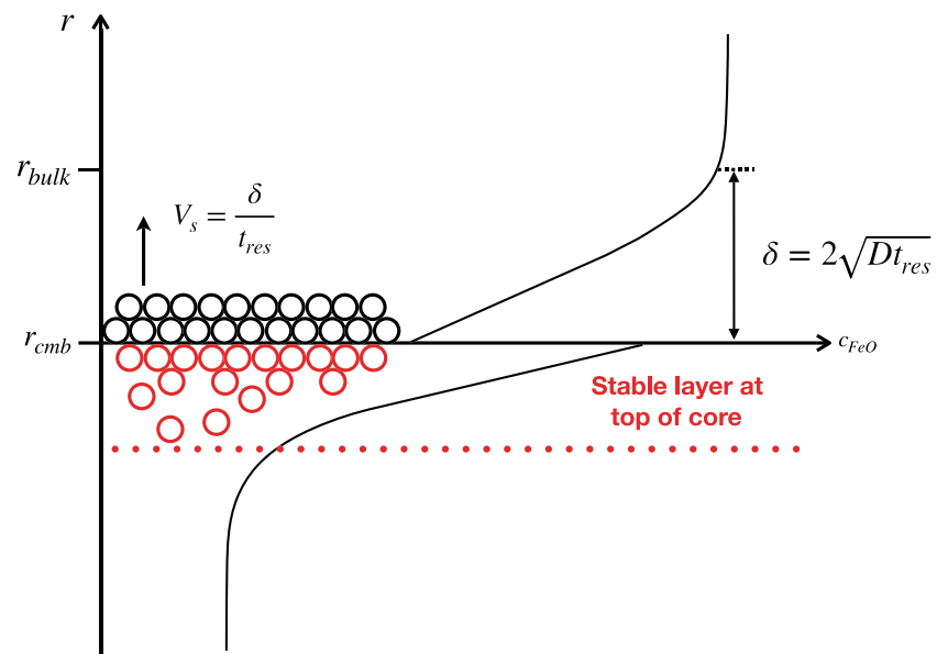
Figure 2. Illustration of chemical exchange between the lower mantle and core. FeO-rich material can be brought into contact with the core by diffusion or buoyancy. Diffusion depletes the lower mantle through a skin depth of thickness \delta = 2\sqrt{Dt_{res}} , where D is the diffusion coefficient and t_{res} the residence time for undepleted material at the core-mantle boundary (CMB). The top of the layer is at radius r_{bulk} and the base of the layer is the CMB radius r_{cmb} . Buoyant FeO-depleted material rises with the Stokes velocity V_s . Passage of FeO across the CMB creates a stably stratified layer (red) at the top of the core.
