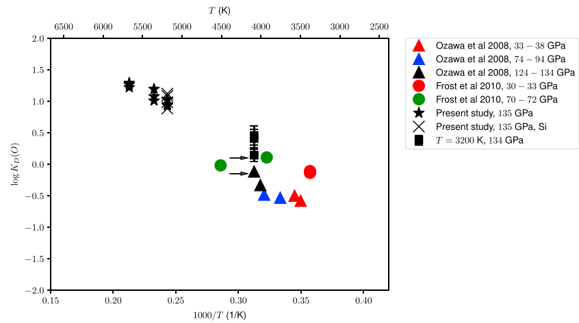
Figure 1. Comparison of our results with published work. Our data are plotted together with other experimental studies of solid silicate-liquid metal partitioning. The arrows highlight the direct comparison discussed in the text between a present calculation and a previous experimental determination of K_D(O) at the same pressure-temperature conditions.
