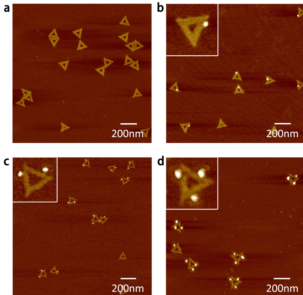
Figure 1. AFM images of triangular DNA origami. (a) pristine origami, (b) functionalized with one QD, (c) functionalized with two QDs, and (d) functionalized with three QDs.
