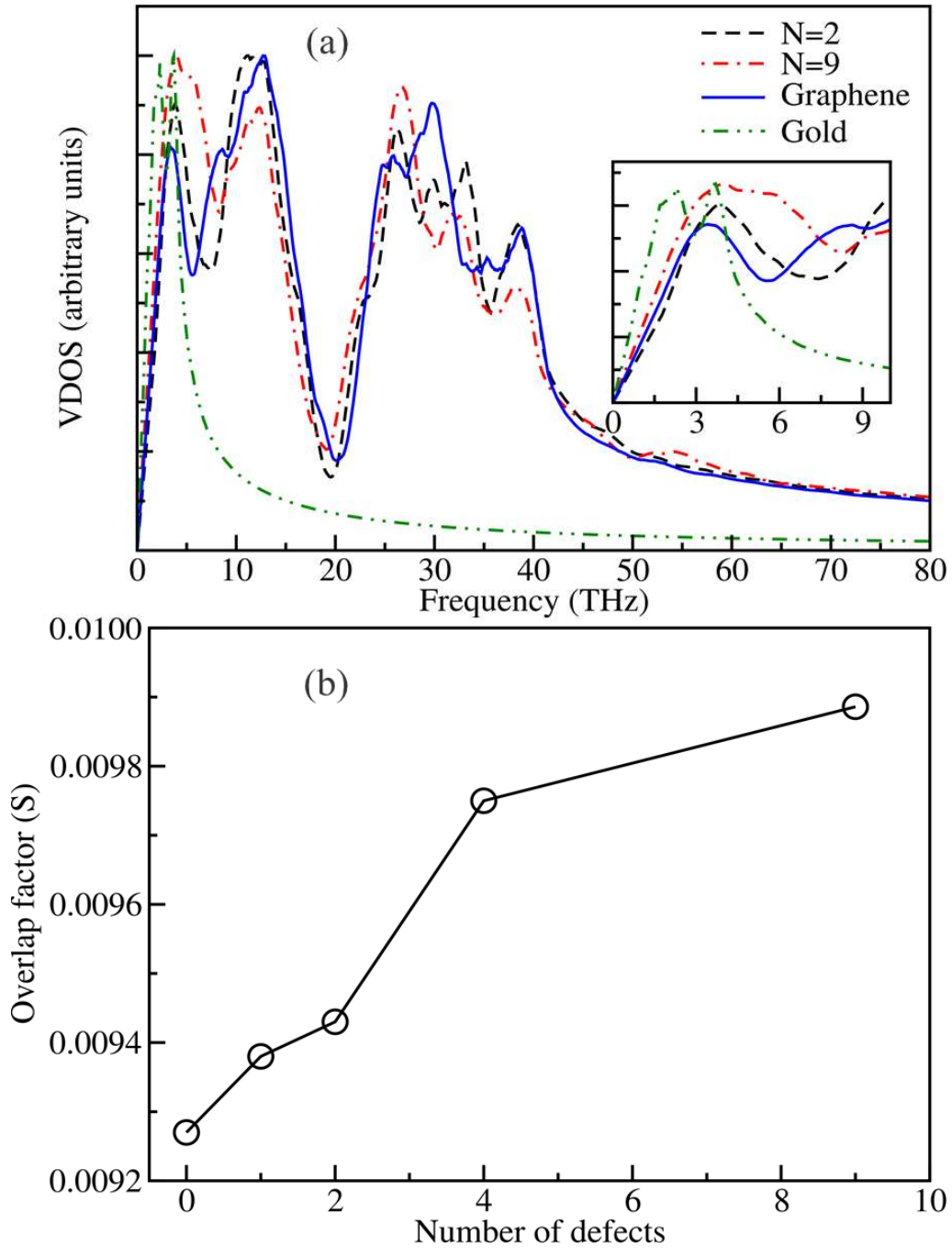
Figure 5. (a) VDOS profiles for defect free graphene, graphene with defects ( N = 2 and 9 ) and gold; The inset shows the zoomed in view of VDOS within 10 THz (b) Variation of gold-graphene VDOS overlap factor with the number of defects in graphene.
