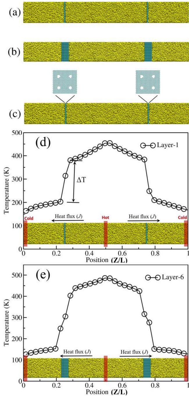
Figure 1. Gold-graphene system with a (a) single graphene sheet (b) graphene of six layers and (c) Graphene sheet with four number of defects; Typical temperature profile within a system of gold-graphene system at 300 K for (d) single layer gold-graphene system and (e) six-layer graphene gold system. The figures shown below the temperature profiles are the model simulation systems used to perform simulations.
