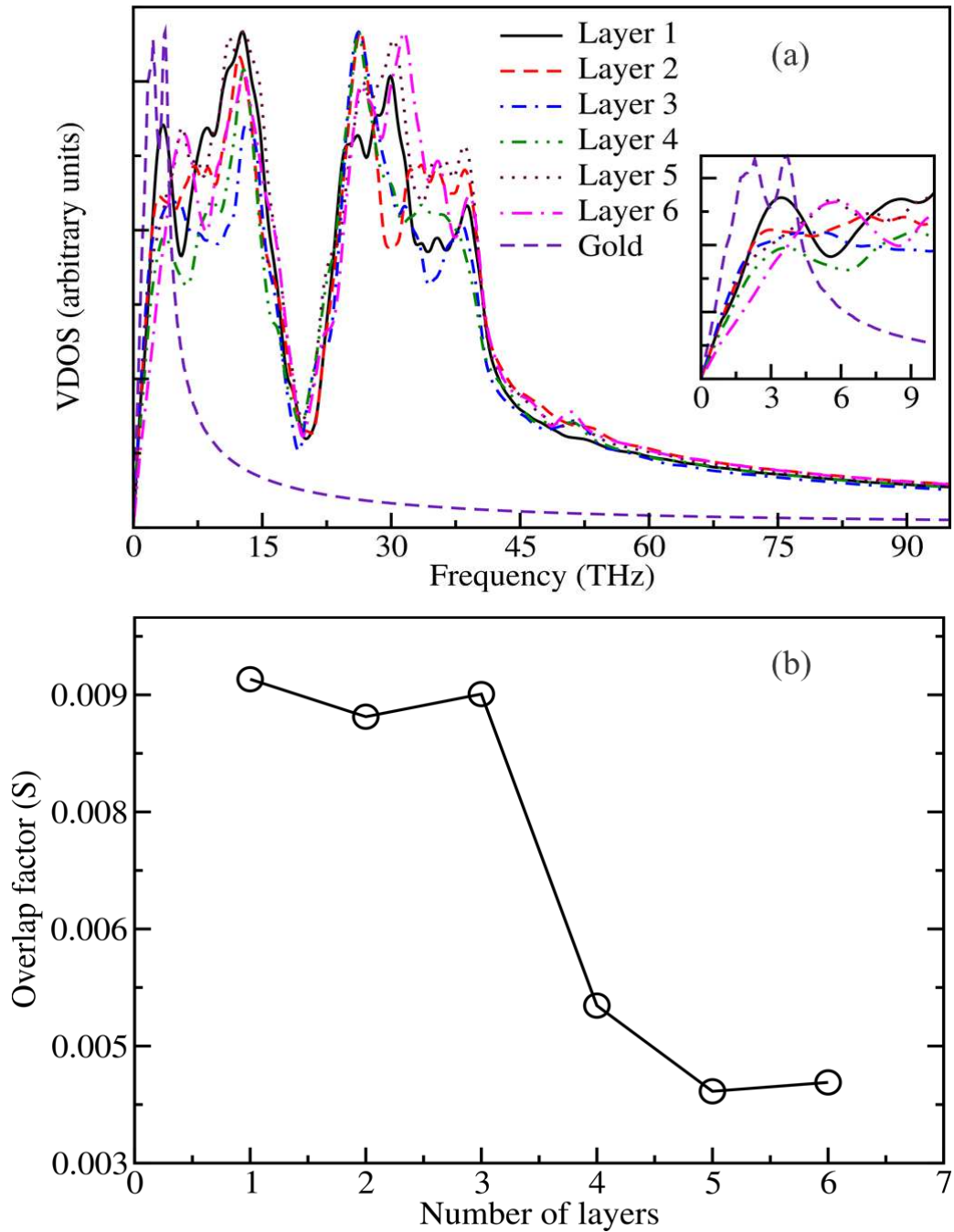
Figure 4. (a) VDOS profiles for n-layer graphene ( n = 1 to 6) and gold (b) Overlap factor obtained for different number graphene layers with gold VDOS.
