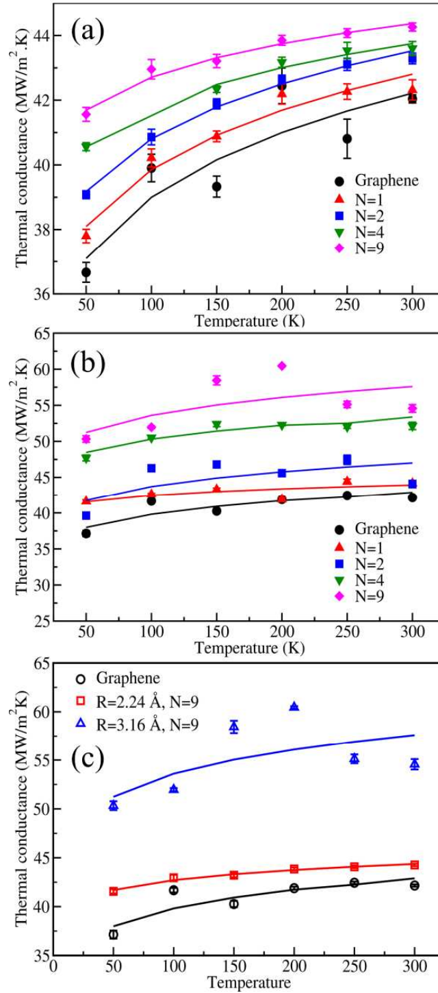
Figure 3. (a) Variation in TC with the temperature and defect density for the case of graphene containing defect of size 2.24 Å, (b) Same as in (a) but with defect of size 3.16 Å and (c) Variation in TC with the temperature and defect size. The solid lines are average trend lines.
