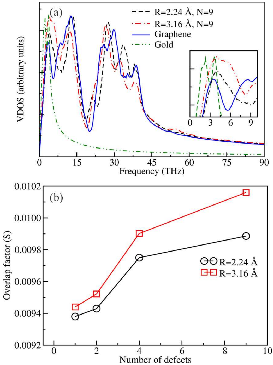
Figure 6. (a) VDOS profiles for gold, defect free graphene and graphene containing 9 defects of size 2.24 and 3.16 Å; inset shows the zoomed in-view of the VDOS within 10 THz (b) Variation of gold-graphene VDOS overlap factor with number of defects in graphene for pore size 2.24 and 3.16 Å.
