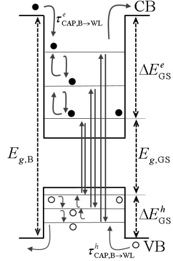
Figure 2: Sketch of the QD sub-band electronic structure highlighting the inter-band and intersubband carrier processes taken into account in the model. E_{g,B} , E_{g,GS} indicate the GaAs and GS bandgap energy, respectively. \Delta E_{GS}^e , \Delta E_{GS}^h the confinement energy for electrons and holes in the GS.
