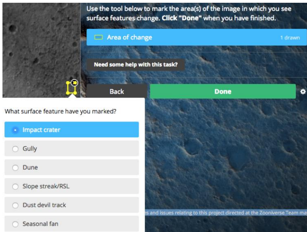
Figure 5 The subtask of feature identification (Step 3 in Figure 1)
