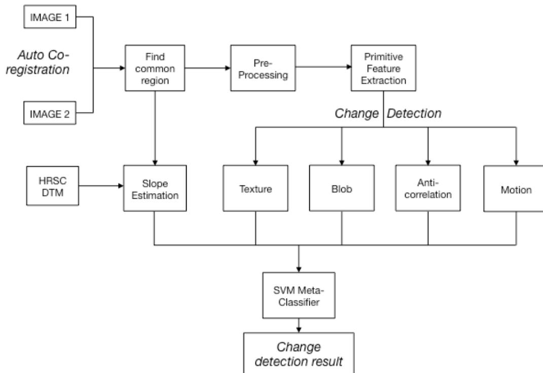
Figure 1 The flowchart of the change detection algorithm. Details of the auto co-registration of image pairs and creation of the High Resolution Stereo Camera Digital Terrain Model (HRSC DTM) are documented in Sidiropoulos and Muller (2016) and Gwinner et al. (2016) respectively.
