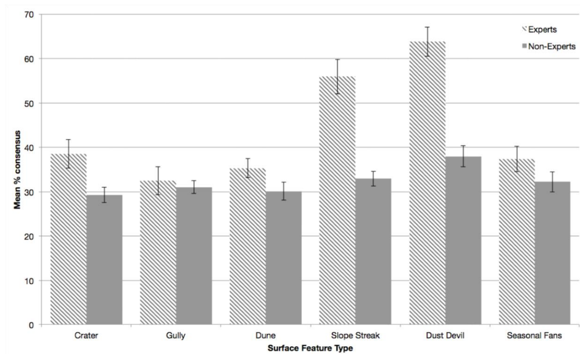
Figure 9 Bar chart comparing the mean % consensus for different surface features between experts (Table 2) and novices (Table 3) with standard error bars to illustrate the significance of differences
