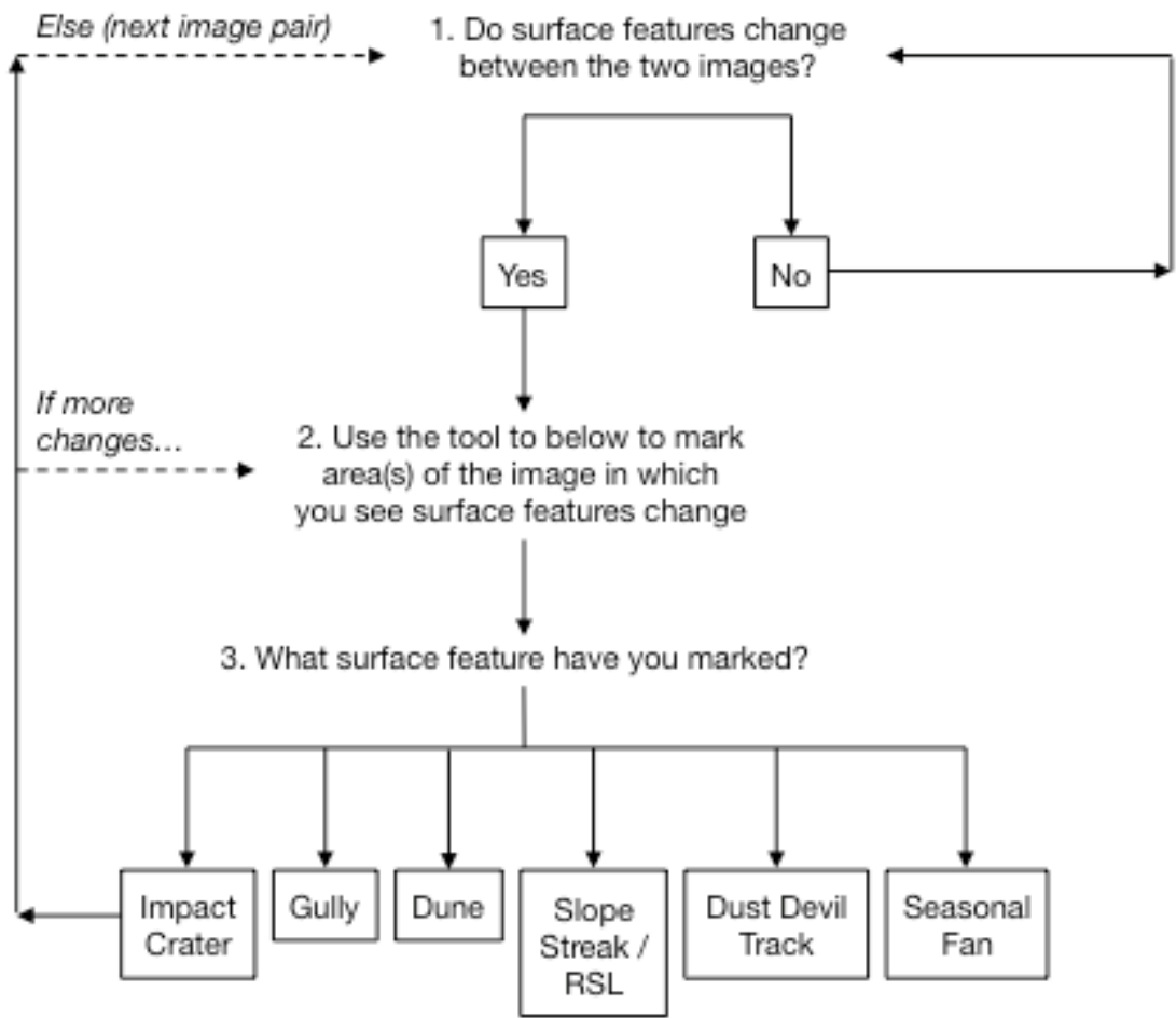
Figure 2 Task workflow: Mars in Motion
