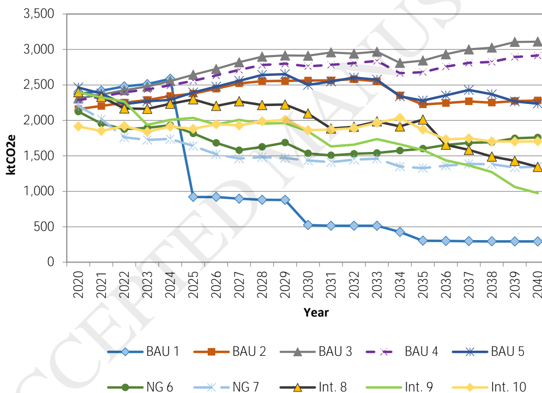
Figure 20. GHG emissions from the power system of Crete
