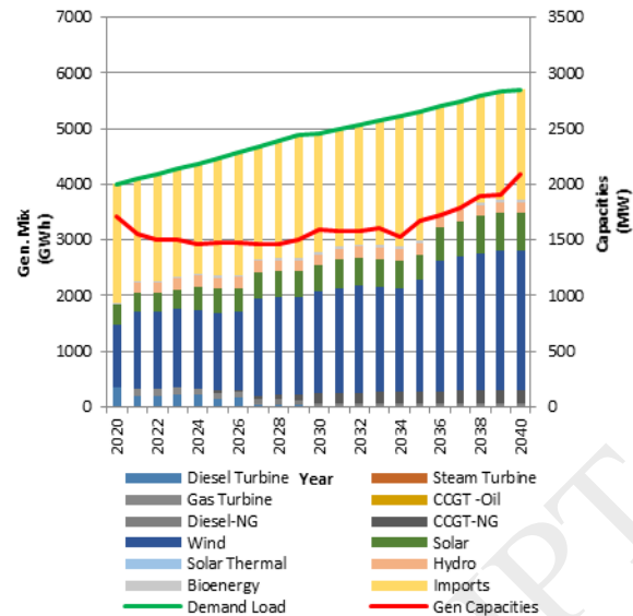
Figure 16. Generation mix for Int. 10
