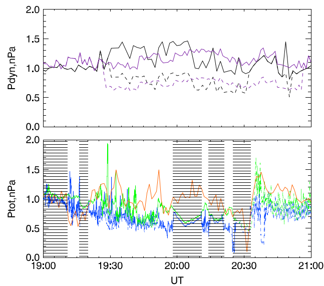
Figure 3. (top) The measured solar wind dynamic pressure from Wind (black, solid) and ACE (violet, solid), and the modified solar wind pressure reduced to 53% in the foreshock region as explained in section 3 (dashed lines). (bottom) The total pressure (the sum of magnetic, thermal, and dynamic pressures) from THB (blue), THC (green), and Geotail (orange). Dashed blue (green) lines show the sum of magnetic and thermal pressures from THB (THC). Time intervals of THB magnetosphere passages are indicated by shadow bars.
