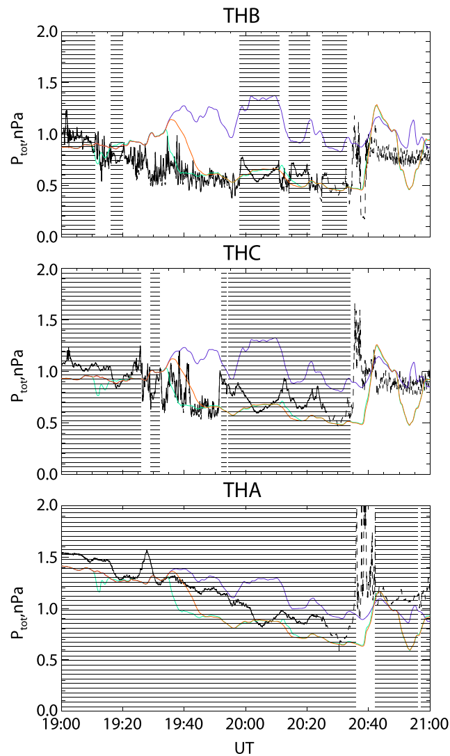
Figure 6. Total (magnetic, thermal, and dynamic) pressures from THEMIS (black), in runs 1 (dark blue), 2 (green), and 3 (red) for the event on 16 July 2007. Dashed black line shows the sum of magnetic and thermal pressures in THEMIS data. Shading indicates THEMIS magnetospheric intervals.
