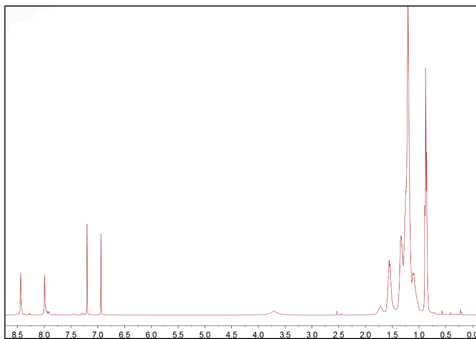
Figure S2. ^1\text{H NMR} spectrum of SiIDT-TPD.
