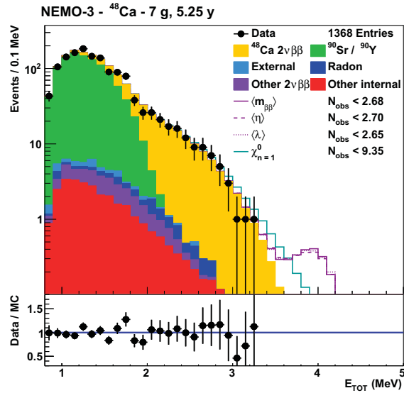
Figure 4. The distribution of the summed electron energy in 2-electron events in ^{48}\text{Ca} . The 2\nu\beta\beta -signal is clearly visible above backgrounds. Open histograms represent limits on non-standard model 0\nu\beta\beta processes. The ratio of data events to the total Monte Carlo prediction is shown in the bottom panel (from [4]).
