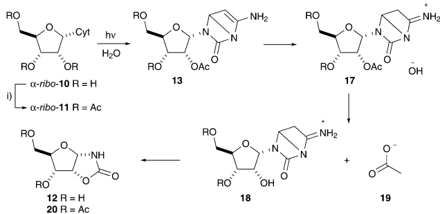
Fig. 5 Photochemical induced ester hydrolysis and oxazolidinone formation upon irradiation of cytidine nucleotides. 15 (i) N -Acetyl imidazole, H 2 O, pH 8, 90%. Cyt = cytosine.
