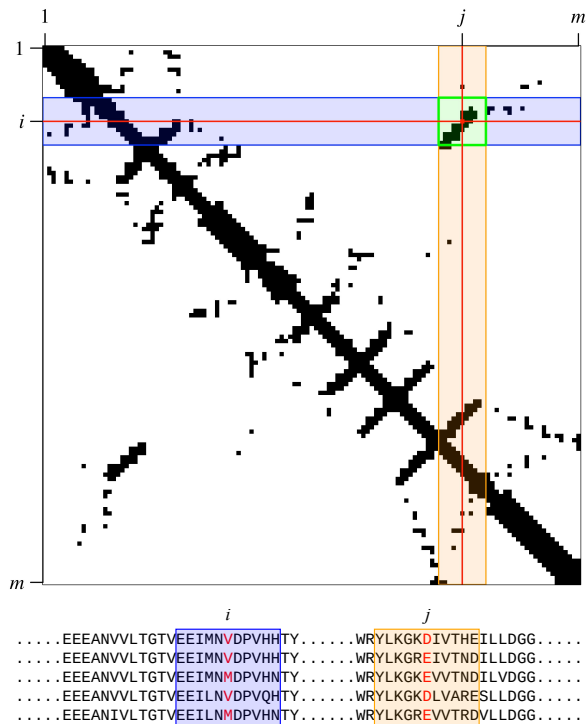
Fig. 2. Illustration of the relationship between alignment columns and data seen by DeepCov during training and inference. The receptive field of DeepCov (green square) is shown on a section of a contact map. The pair frequency or covariance matrices used as input to the network have the same dimensions as the contact map ( m \times m ), and DeepCov learns the relationship between the two. As the receptive field moves across the input matrix, it sees a different subset of the input, and this corresponds to a different set of columns in the input alignment (bottom). In this example, the residue pair i, j (shown in red) is being evaluated for the presence of a contact, and the receptive field of DeepCov is set to 11, meaning that windows of 11 residues centred on residues i and j are considered during training and prediction (shaded blue and orange, respectively). Only the sequence data in these windows (and hence the sections in the input and output matrices covered by the receptive field in green) are used when learning the relationship between sequence data and the presence or absence of a contact between residues i and j .
