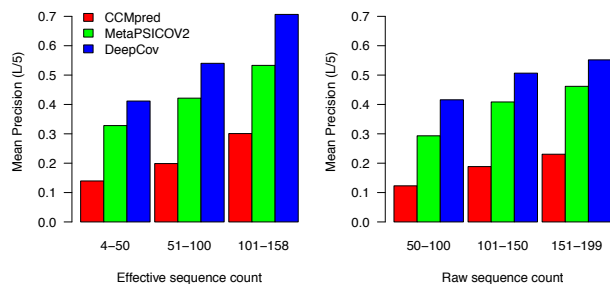
Fig. 4. Comparison of performance on 232 shallow alignments. Mean precision for the top-L/5 contacts are plotted as a function of alignment depth for CCMpred, MetaPSICOV2 and DeepCov. Raw and effective sequence counts are binned into three categories. DeepCov achieves higher precision than CCMpred and MetaPSICOV2 on small protein sequence families. Similar trends are seen when considering the top-L, L/2 and L/10 contacts.
