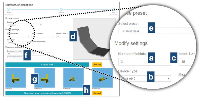
Figure 14. GUI tool for creating customized workspaces.
