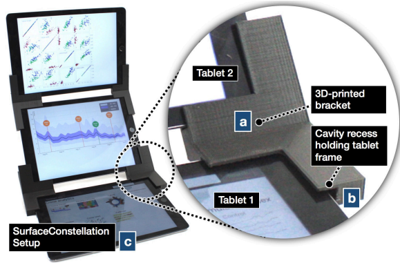
Figure 2. Basic SurfaceConstellation bracket design.
