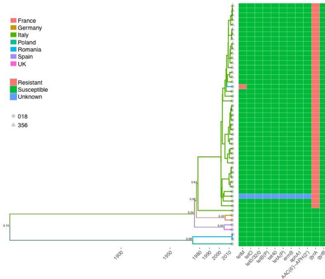
Figure S1. Combined ribotype-018 and ribotype-356 phylogeny with ancestral country reconstruction and antimicrobial resistance determinants. The tree tips are annotated with a circle (ribotype-018) or a triangle (ribotype-356).
