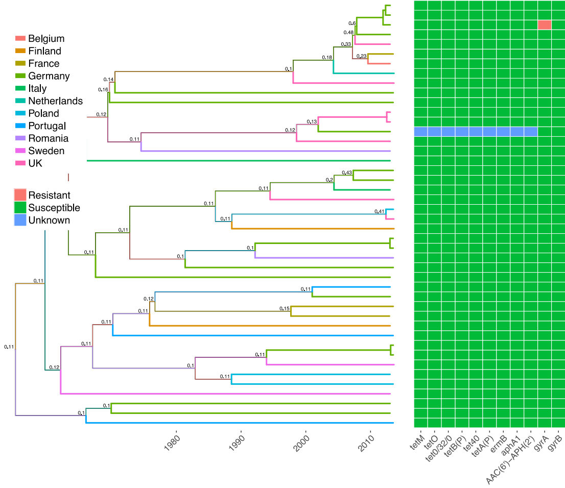
Figure S4. Ribotype-002 phylogeny with ancestral country reconstruction and antimicrobial resistance determinants
