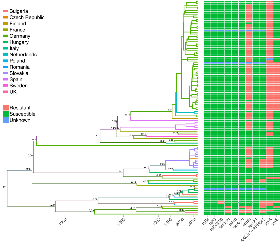
Figure S2. Ribotype-001 phylogeny with ancestral country reconstruction and antimicrobial resistance determinants.
