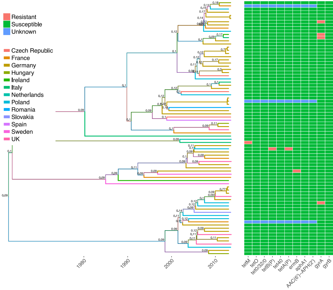
Figure S5. Ribotype-014 phylogeny with ancestral country reconstruction and antimicrobial resistance determinants.
