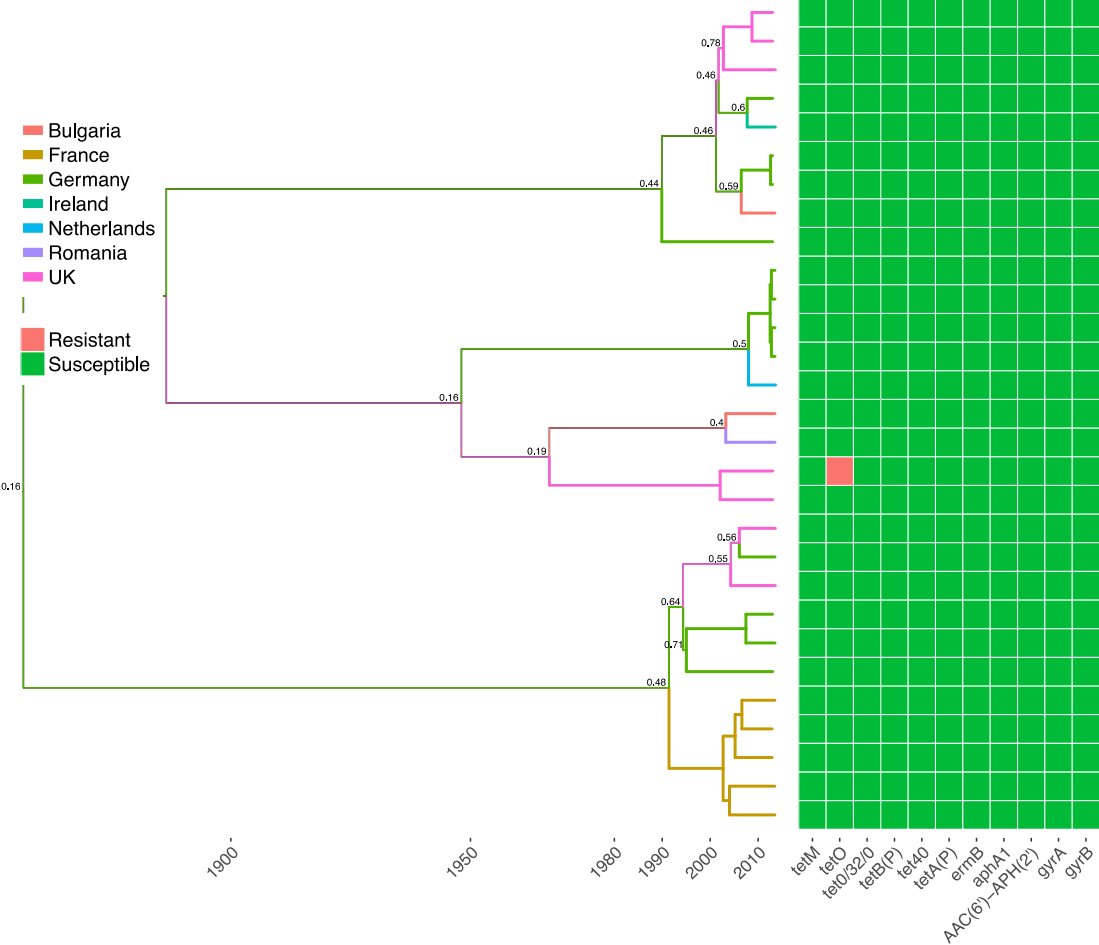
Figure S6. Ribotype-015 phylogeny with ancestral country reconstruction and antimicrobial resistance determinants.
