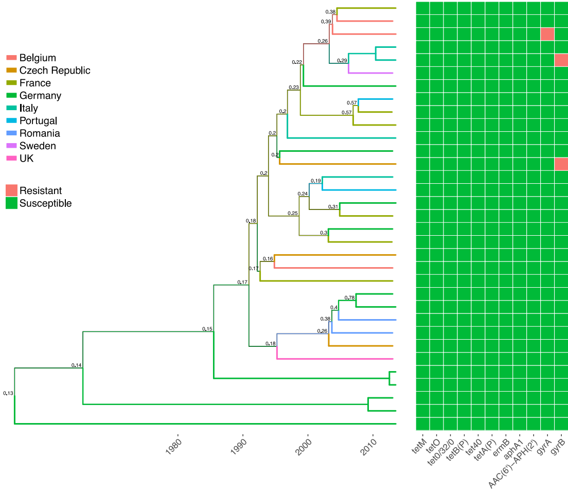
Figure S7. Ribotype-020 phylogeny with ancestral country reconstruction and antimicrobial resistance determinants.
