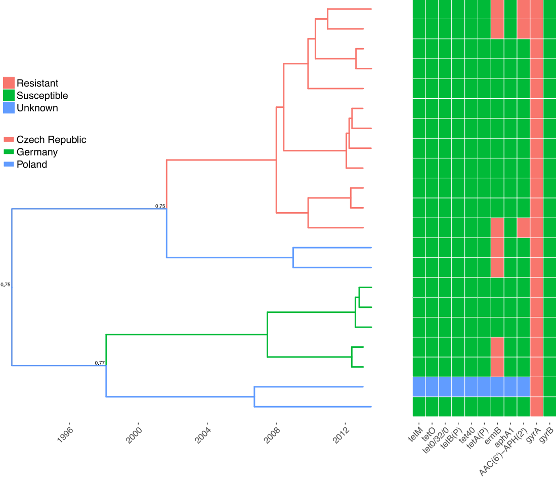
Figure S3. Ribotype-176 phylogeny with ancestral country reconstruction and antimicrobial resistance determinants.
