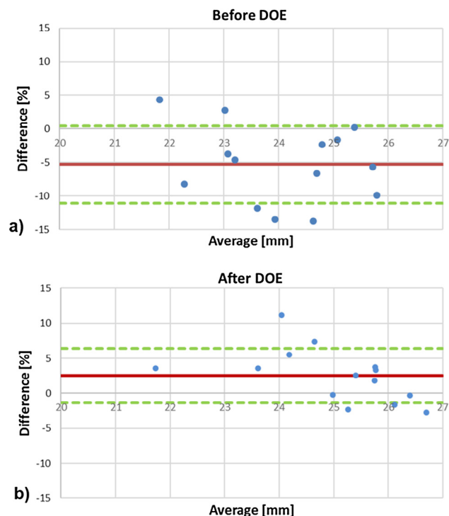
Fig. 4. Bland Altman plots for the comparison between stent diameters measured from fluoroscopy images and computational results before (a) and after (b) refinement of the material parameters: the red line represents the mean difference and the green dashed lines \pm standard deviations. (For interpretation of the references to colour in this figure legend, the reader is referred to the web version of this article.)
