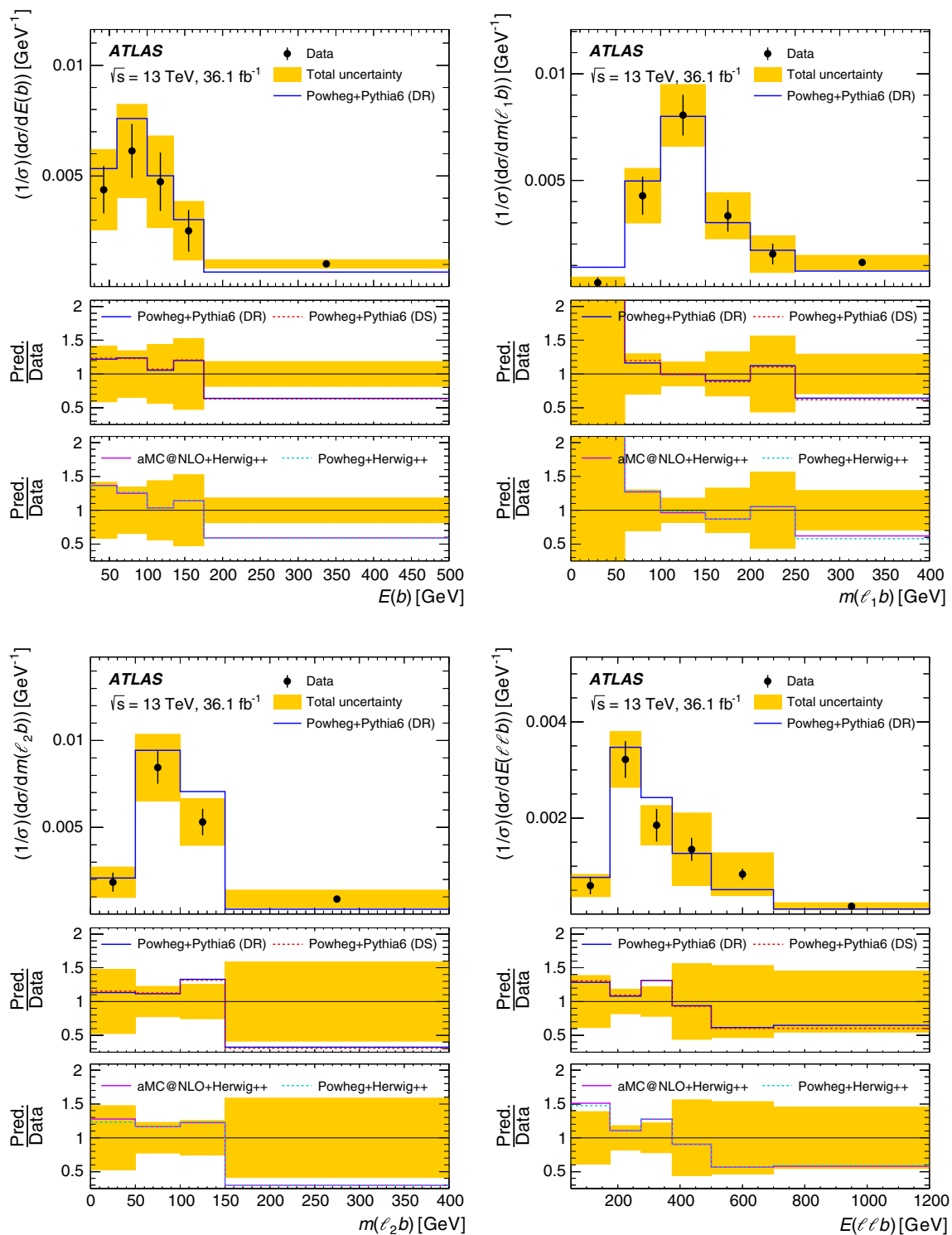
Fig. 5 Normalised differential cross-sections unfolded from data, compared with selected MC models, with respect to E(b) , m(\ell_1b) , m(\ell_2b) , and E(\ell\ell b) . Data points are placed at the horizontal centre of each bin, and the error bars on the data points show the statistical uncer-
