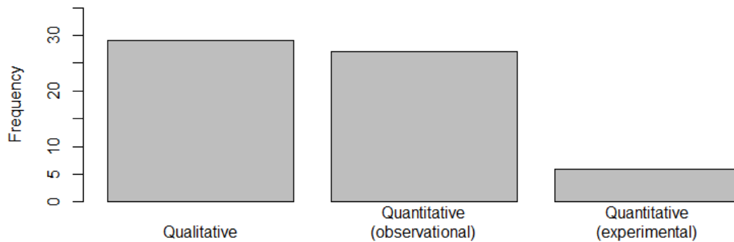
Figure A3: Studies by method
