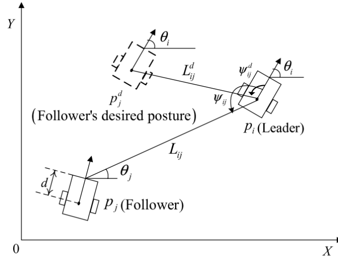
Fig. 6: Leader-follower formation control approach. Formation is maintained by keeping the desired distance and angle between the leader and each follower 47 .
