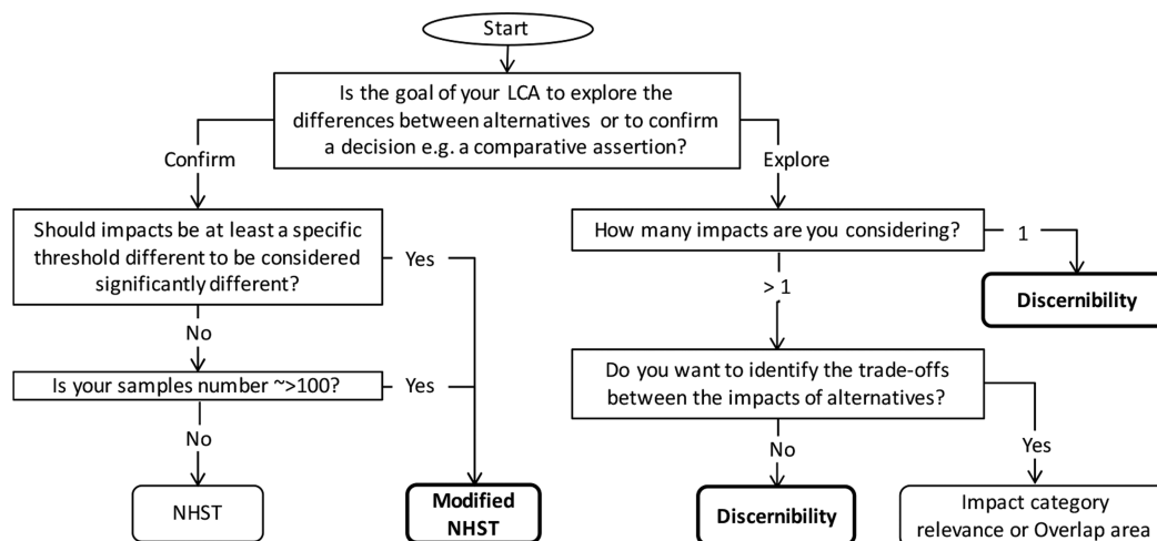
Figure 3. Decision tree to guide LCA practitioners on which uncertainty-statistics method (USM) to use for the interpretation of propagated LCA uncertainty outcomes in comparative LCAs. Thicker lines indicate recommended methods for confirmatory and exploratory purposes as per the considerations described in the main text. The type of information available from the uncertainty analysis results (in the following parentheses) determines the choice between impact category relevance (statistical parameters of the distributions) or overlap area (MC runs).
