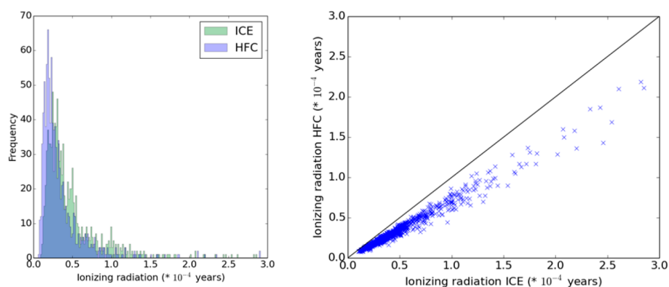
Figure 2. Histograms (left) and scatter plot (right) for 1000 MC runs for the hydrogen fuel cell (HFC) vehicle and the internal combustion engine (ICE) vehicle for ionizing radiation. The performances of ICE and HFC show great similarities in the histogram, and thus a large overlap area (i.e., 0.79). However, the scatter plot shows that for each MC run, the difference between HFC and ICE \neq 0 (the diagonal line in the scattered plot represents equal values for both alternatives). Hence, alternatives are discernible in 100% of the runs.
