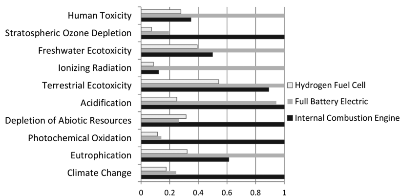
Figure 1. Deterministic results (scaled to the maximum results per impact) for comparative LCA of three alternatives of vehicles.
