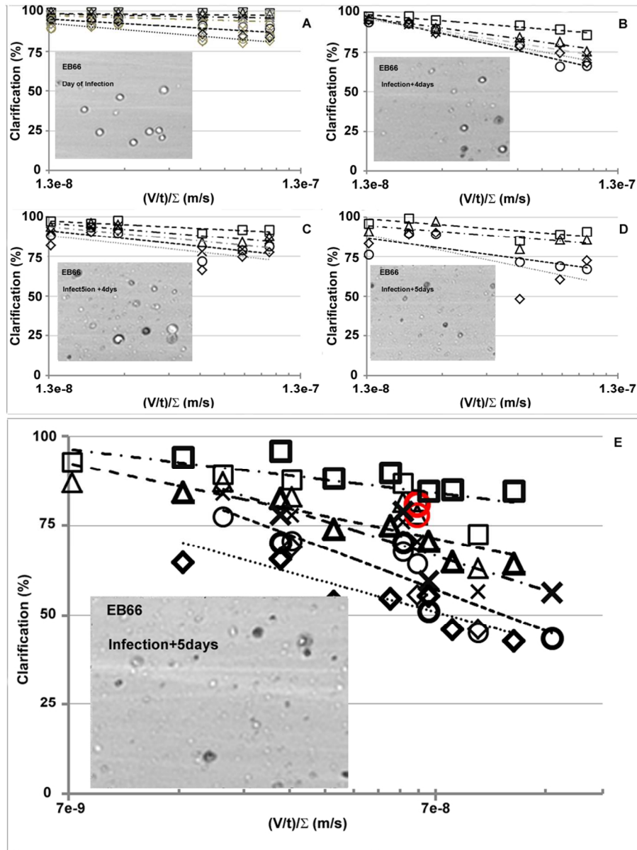
Normalised clarification of EB66 cells, (A) uninfected with influenza virus, (B,C) infected with influenza virus for 4 days and (D) infected with influenza virus for 5 days. Cells have been subjected to disruption by a rotating shear device at varying shear rates prior to clarification in a laboratory centrifuge, with rotating shear device speeds of 0krpm (squares), 6krpm (triangles), 8krpm (crosses), 10krpm (circles) and 12krpm (diamonds) respectively. Measurements shown are for a single representative run (as all influenza runs used different viral strains), with the exception of (A), where triplicate results are shown. Normalised clarification of EB66 cells, infected with flu virus for 5 days, where cells have been subjected to disruption by a rotating shear device at varying shear rates prior to clarification in a Beckmann laboratory centrifuge, using 15ml falcon tubes, with rotating shear device speeds of 0krpm (squares), 6krpm (triangles), 8krpm (crosses), 10krpm (circles) and 12krpm (diamonds) respectively (E). Measurements shown in E are for two separate runs, each using a different viral strain of influenza. In addition red circles give the clarification measured on the PSC-5 centrifuge.
