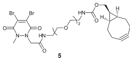
Fig. 2 Structure of PD-based re-bridging reagent.
