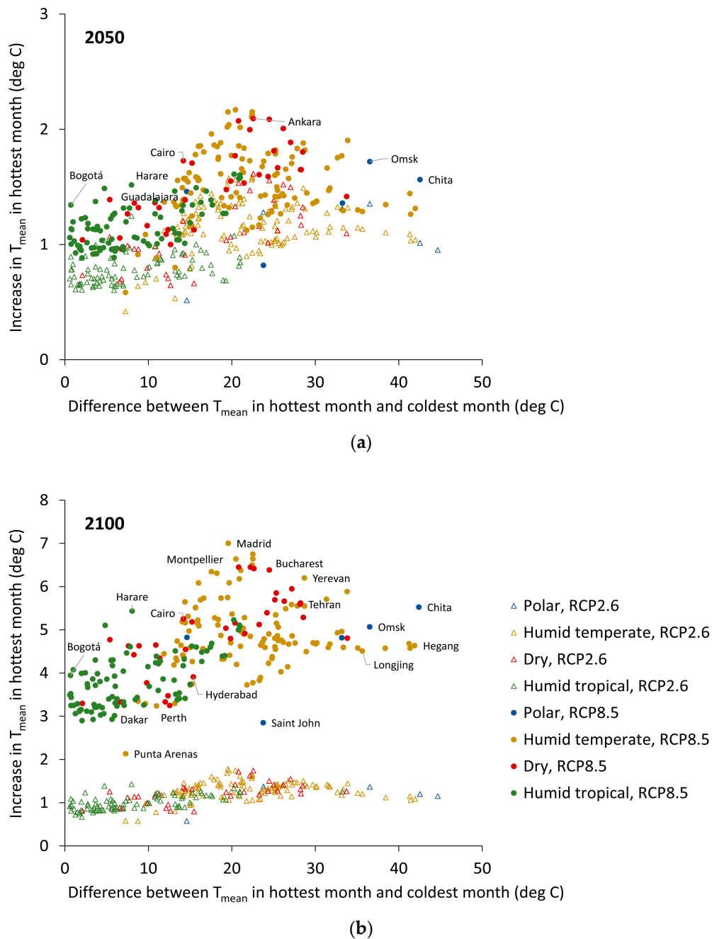
Figure 5. Increases in T_{mean} for the hottest month relative to 2017: relationship to the seasonal variation in temperature as represented by the difference between the T_{mean} for the hottest and coldest month by (a) the year 2050 and (b) the year 2100. Colouring indicates Bailey’s ecoregion domain.
