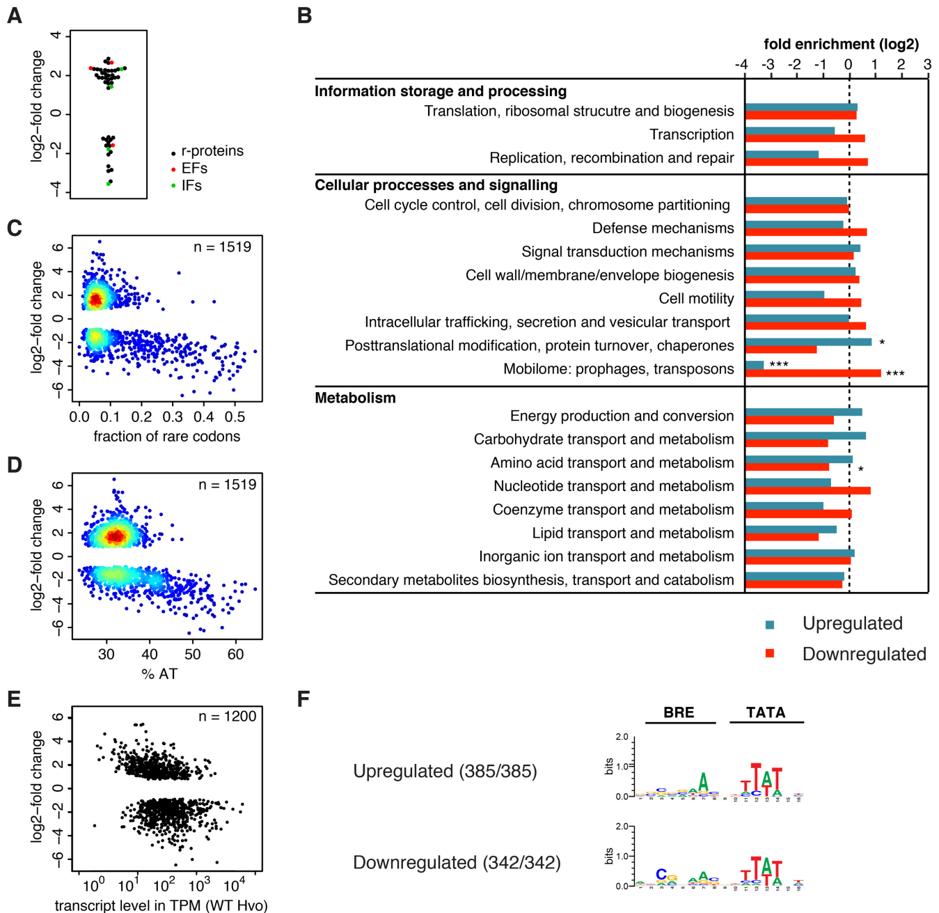
Figure 6. Deletion of tfeB leads to widespread misregulation of transcription. (A) log 2 -fold change in relative transcript abundance ( P_{\text{adj}} < 0.01 ) of genes coding for the basal translation machinery, ribosomal proteins (black), translation initiation factors (green) and elongation factors (red). (B) Analysis arCOG category distribution in significantly misregulated genes ( P_{\text{adj}} < 0.01 ). Significant enrichment or underrepresentation is indicated (two-sided Fisher's exact test with Bonferroni correction for multiple testing) with * and *** denoting P_{\text{adj}} < 0.05 and 0.001 , respectively. (C and D) Heatscatter plot of rare codon frequency (defined as codons with less than 10% synonymous codon usage genome-wide) (C) and AT content of genes (D) against the log 2 -fold change ( P_{\text{adj}} < 0.01 ) in relative transcript abundance. (E) Plot showing the estimated transcript levels in parental strain H26 (transcripts per million, TPM, geometric mean for the two replicates) calculated for the transcription units of Hvo using RSEM (31) against the log 2 -fold change in relative transcript abundance for the first cistron within the respective transcription unit ( P_{\text{adj}} < 0.01 ). (F) BRE/TATA motif consensus in misregulated genes. In order to account for variable spacing between the TSS and BRE/TATA motifs we conducted a motif search using the MEME software version 4.11.4 (0 or 1 occurrence per sequence, 4 to 16 bp width, searching given strand only) (33). A background model based on the composition of the combined H. volcanii DS2 genome was employed. BRE/TATA motifs were discovered in all sequences.
