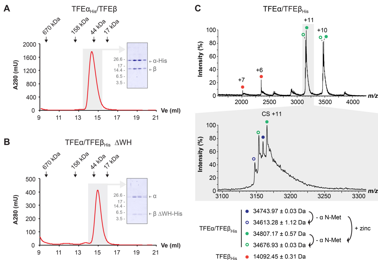
Figure 2. Hvo TFE \alpha and TFE \beta form a dimeric complex in the absence of an FeS cluster. (A and B) Size exclusion chromatography of TFE \alpha_{His} /TFE \beta (A) and TFE \alpha /TFE \beta_{His} \Delta WH (B) on a superose 12 h 10/30 column. Elution peaks of standard proteins are indicated. Peak fractions (highlighted in gray) were subjected to SDS-PAGE and Coomassie-staining (insert) to show symmetric elution of both subunits. (C) nESI mass spectrum of TFE \alpha /TFE \beta_{His} . The different charge state series observed are labelled with red, blue and green filled circles. Charge state series derived from additional cleavage of TFE \alpha N-Met are labelled with open circles. Highlighted in gray is a zoom over the region that includes charge state (CS) +11. All detected masses indicate the absence of a cubane 4Fe-4S cluster (352 Da).
