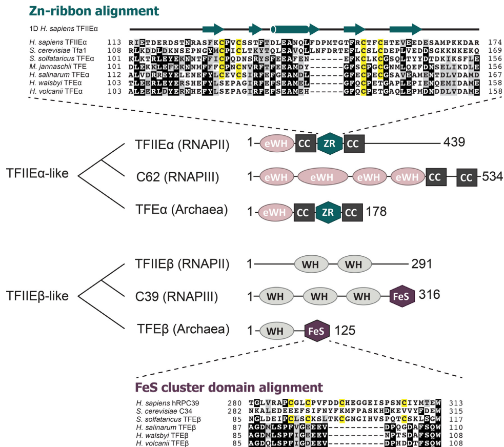
Figure 1. Overview over the domain organization of archaeal TFE subunits and related eukaryotic proteins. TFE \alpha -related proteins are composed of extended winged-helix domains (eWH), a zinc ribbon domain (ZR) and coiled coil (CC) (3–5,55). TFE \beta -related proteins are composed of winged-helix (WH) and iron-sulphur cluster domains (FeS). Sequence alignments of the two metal binding domains (ZR and FeS) reveal the loss of cysteine residues (highlighted in yellow) required for metal coordination in H. volcanii TFE \alpha and TFE \beta . Key to sequences: H. sapiens TFII \alpha (NCBI accession: P29083), S. cerevisiae Tfa1 (EDN59878), S. solfataricus TFE \alpha (AAK40605), M. jannaschii TFE (Q58187), H. salinarum TFE \alpha (AAG19231), H. walsbyi TFE \alpha (ERG94676), H. volcanii TFE \alpha (ELK55987), H. sapiens C39 (EAX10240), S. cerevisiae C34 (P32910), S. solfataricus TFE \beta (AAK41220), H. salinarum TFE \beta (WP_010902769), H. walsbyi TFE \beta (ERG96516), H. volcanii TFE \beta (ADE03923). The secondary structure of the H. sapiens TFII \alpha ZR domain is based on Okuda et al. (43).
