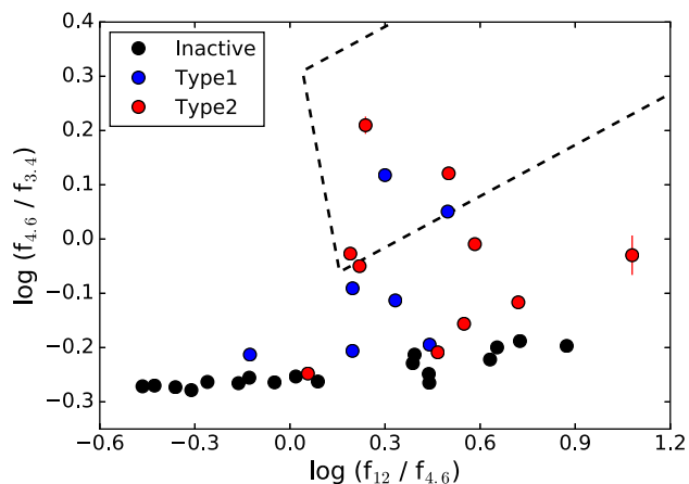
Figure 4. LLAMA galaxies plotted on the WISE colour–colour diagram of Mateos et al. (2012), with the ratio of W3 (12 \mu\text{m} ) to W2 (4.6 \mu\text{m} ) fluxes on the x-axis and W2 to W1 (3.4 \mu\text{m} ) fluxes of the y-axis. AGN are shown with blue (Type 1) and red (Type 2) points, and inactive galaxies with black points. Error bars are plotted, but may be too small to be visible. The dashed lines delineate a region of the diagram which contains objects with a MIR SED dominated by AGN torus emission.
