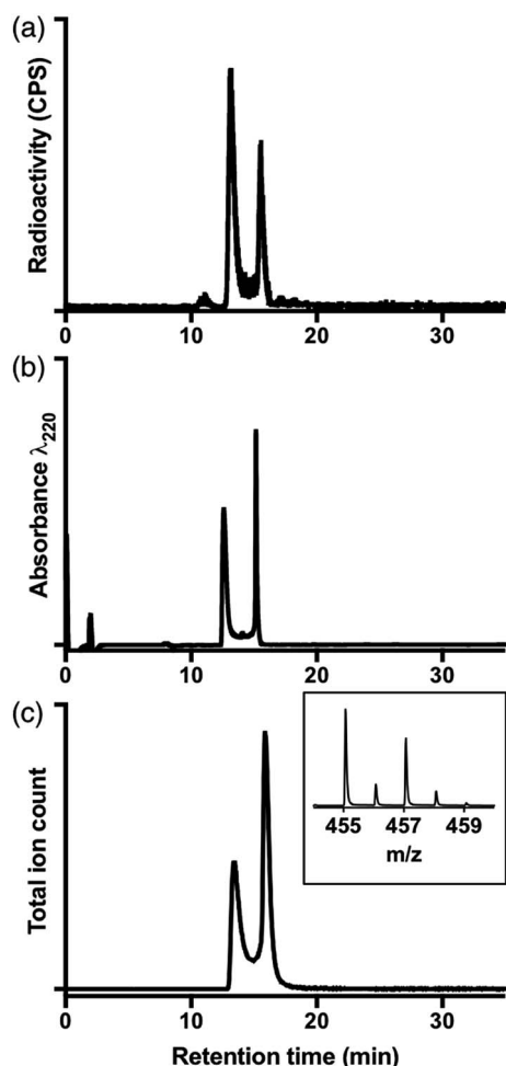
Fig. 4 (a) Radiochromatogram of [ ^{68}\text{Ga}(\text{HBED}) ] (prepared at 90^\circ\text{C} ); (b) UV chromatogram of [ \text{Ga}(\text{HBED}) ]; (c) extracted ion chromatogram of isolated [ \text{Ga}(\text{HBED}) ] ( m/z of monoisotopic signal = 455.07); inset positive ion MS spectrum of \{[\text{Ga}(\text{HBED})] + 2\text{H}^+\} : [\text{Ga}(\text{C}_{20}\text{H}_{22}\text{N}_2\text{O}_6)]^+ .
