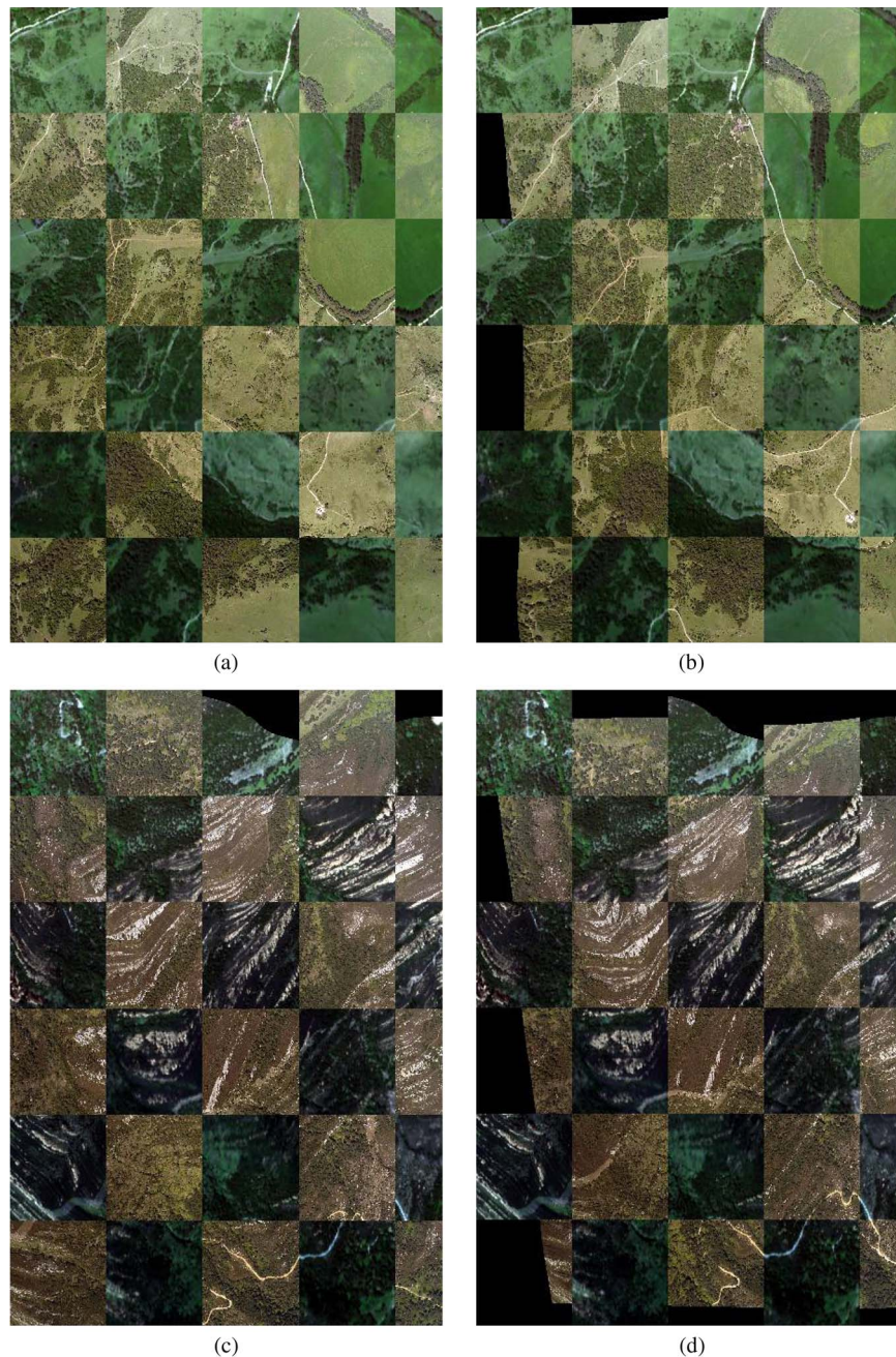
Fig. 5. Checkerboard overlay between aerial photograph template images T and hyperspectral reference images R and checkerboard overlay of registered aerial photograph template images ( T_{\text{reg}}^{\text{NGF-Curv}} ) and hyperspectral reference images ( R ) generated by our NGF-Curv approach. (a) and (b) Flat terrain case. (c) and (d) Rugged terrain case.
