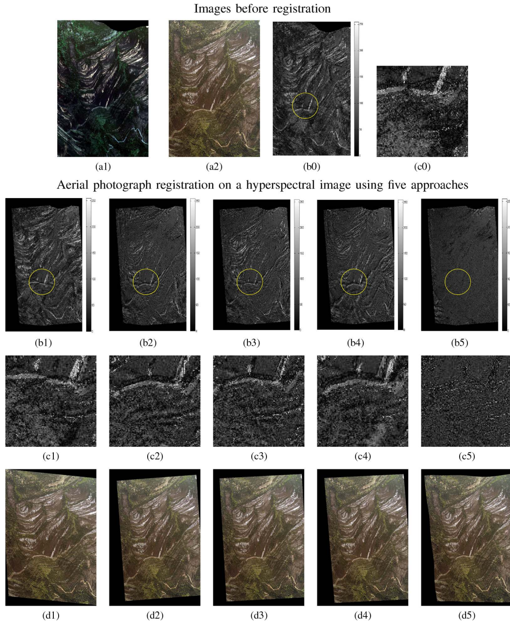
Fig. 4. Image registration of an aerial photograph onto a hyperspectral image in the case of rugged terrain (scale 2400 \times 1800 \text{ m}^2 ). The first row shows (a1) a hyperspectral reference image R ; (a2) an aerial photograph template image T ; the second row shows (b0) a map of difference between these images (i.e., |T - R| ) for methods NCC, MI, NGF, SURF, and NGF-Curv. The third row (c0) zooms in on the circular regions of (b0). The last row of panels shows the aerial photograph template image after it has been registered using methods (d1) NCC, (d2) MI, (d3) NGF, (d4) SURF, and (d5) NGF-Curv.
