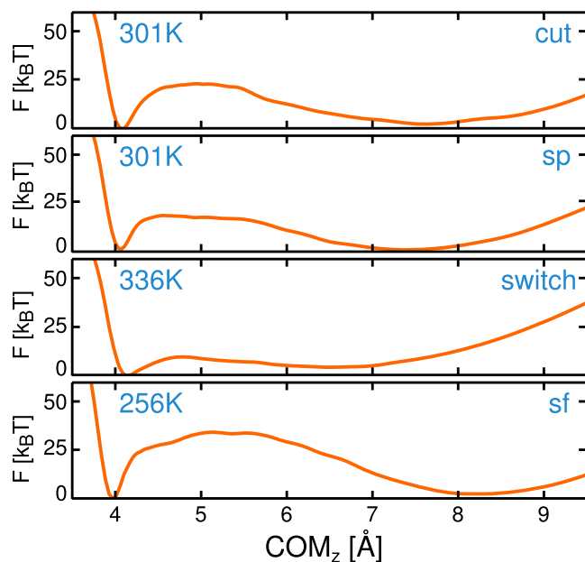
FIG. 3. Free energy profiles of wetting approximately at the transition temperature with uncorrected setup (cut) and for different correction schemes [shifted potential (sp), force switch (switch), and shifted force (sf)] applied with a cutoff at 3\sigma . None of the schemes show the correct behavior, which is shown in Fig. 2 to be a single basin.
