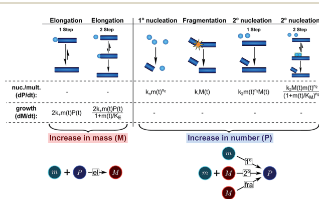
Fig. 3 Processes of fibrillar self-assembly. The processes that make up the reaction network of filamentous self-assembly fall into two categories, nucleation/multiplication processes, which produce new fibril ends, P , and only a negligible quantity of new fibril mass, and growth processes, which produce fibril mass, M , but leave the fibril number unchanged. The contributions to the rates of growth and nucleation/multiplication are given below the schematic representation for each process. For elongation and secondary nucleation we use two alternative schemes, a single-step and a two-step one. Under certain conditions the single-step description may be sufficient, as discussed in the main text. The rate constants and reaction rates are defined in Table 1.
