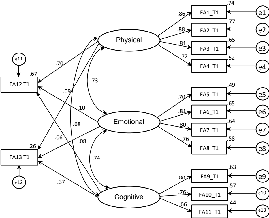
Figure 1: Graphical presentation of the confirmatory analysis (previous model)
