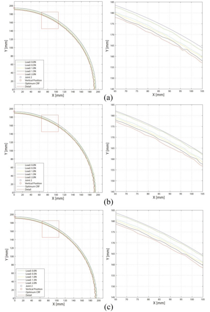
Figure 5 - End effector position in the XY plane (defined as best fit plane for the sequential position of the end effector) when actuating J3 from 0° to 90° when the pressure inside the VSLs are (a) 0Bar, (b) 1 Bar and (c) 2 Bar. In all graphs, the data is plotted for different load levels on the end effector (0N, 0.5N, 1N, 1.5N and 2N). The reference system is centered in J3. During the experiments, the VSL1 is kept in vertical position; The pressure level of VSL1 and VSL2 is identical. J3 was actuated at a speed of 30°/s.
